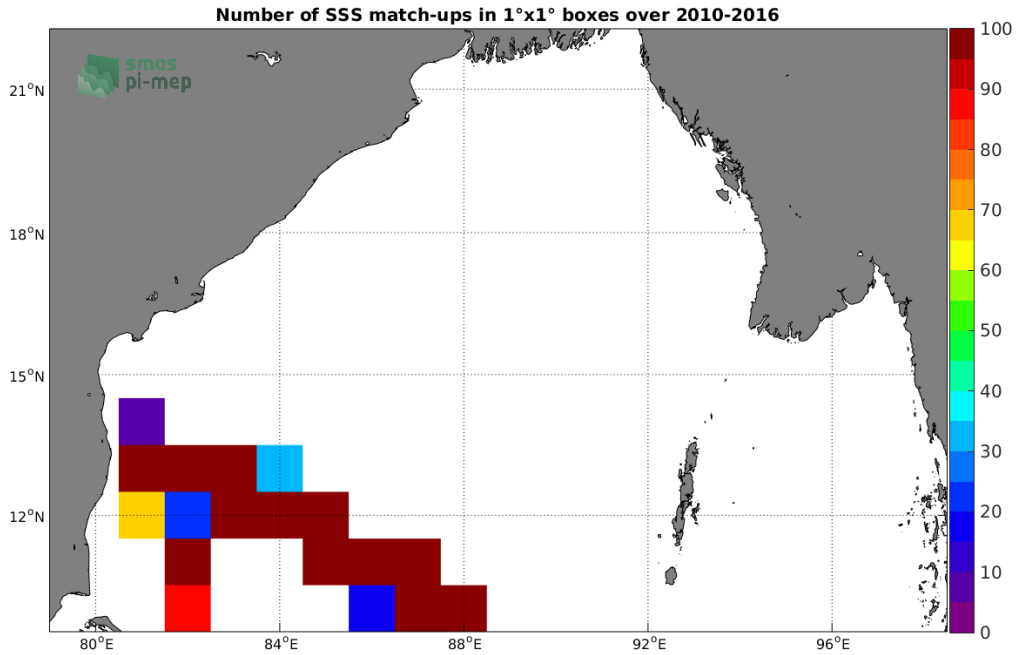
Figure 4: Number of SSS match-ups between TSG (LEGOS-DM) SSS and the SMOS SSS L3 v5 - 9 Days (CATDS-CECOS-LOCEAN) SSS product for the Bay of Bengal Pi-MEP region over 1^\circ \times 1^\circ boxes and for the full satellite product period.
