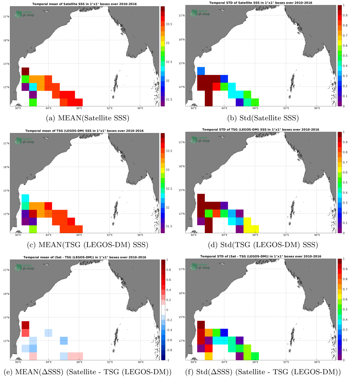
(e) MEAN( \Delta SSS) (Satellite - TSG (LEGOS-DM)) (f) Std( \Delta SSS) (Satellite - TSG (LEGOS-DM)) Figure 6: Temporal mean (left) and Std (right) of SSS from SMOS SSS L3 v5 - 9 Days (CATDS-CECOS-LOCEAN) (top), TSG (LEGOS-DM) (middle), and of \Delta SSS (Satellite - TSG (LEGOS-DM)). Only match-up pairs are used to generate these maps.
