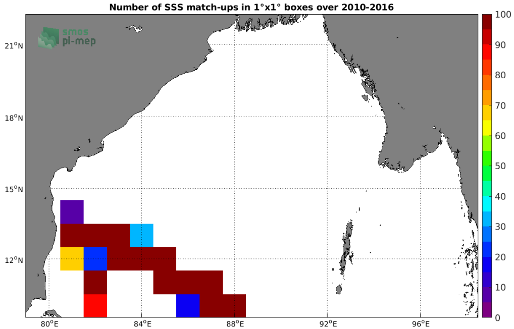
Figure 4: Number of SSS match-ups between TSG (LEGOS-DM) SSS and the SMOS SSS L3 v5 - 18 Days (CATDS-CECOS-LOCEAN) SSS product for the Bay of Bengal Pi-MEP region over 1^\circ \times 1^\circ boxes and for the full satellite product period.
