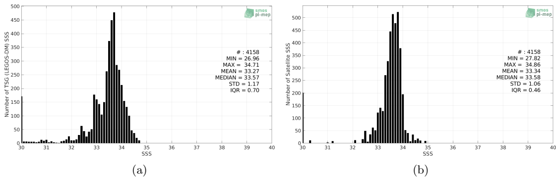
Figure 2: Histograms of SSS from TSG (LEGOS-DM) (a) and SMOS SSS L3 v5 - 18 Days (CATDS-CECOS-LOCEAN) (b) considering all match-up pairs per bins of 0.1 over the Bay of Bengal Pi-MEP region and for the full satellite product period.
