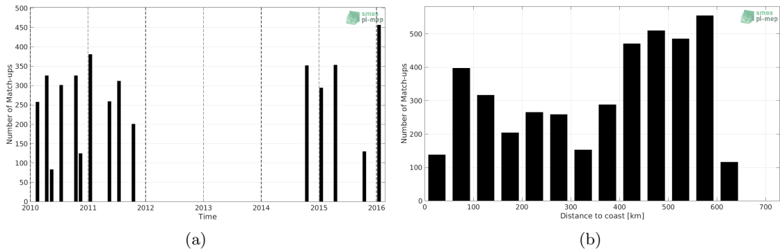
Figure 1: Number of match-ups between TSG (LEGOS-DM) and SMOS SSS L3 v5 - 18 Days (CATDS-CECOS-LOCEAN) SSS as a function of time (a) and as function of the distance to coast (b) over the Bay of Bengal Pi-MEP region and for the full satellite product period.
