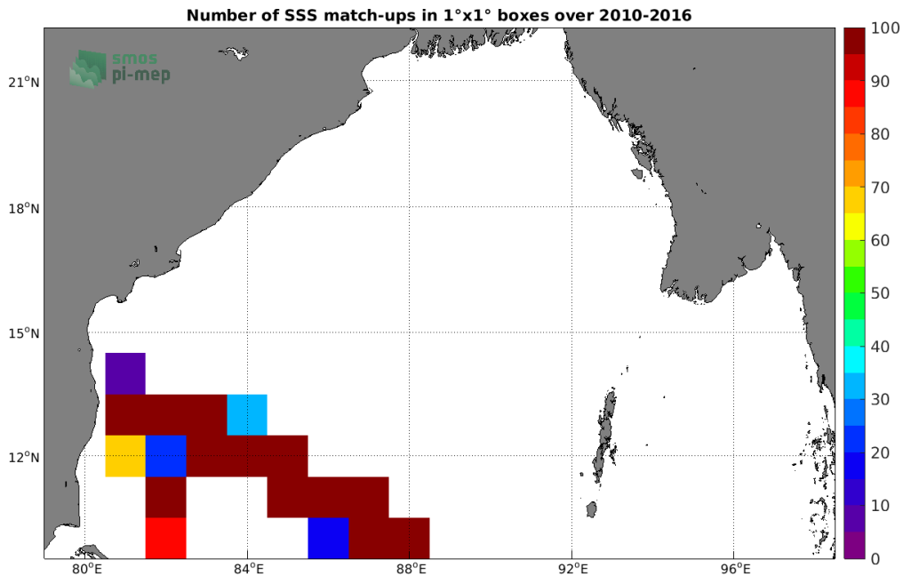
Figure 4: Number of SSS match-ups between TSG (LEGOS-DM) SSS and the SMOS SSS L3 v5 - 18 Days (CATDS-CECOS-LOCEAN) SSS product for the Bay of Bengal Pi-MEP region over 1°x1° boxes and for the full satellite product period.
