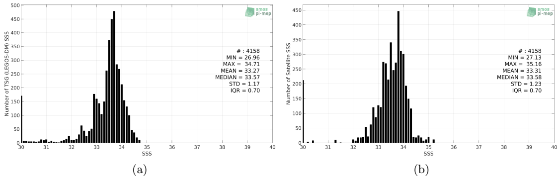
Figure 2: Histograms of SSS from TSG (LEGOS-DM) (a) and SMOS SSS L3 v4 - 9 Days (CATDS-CECOS-LOCEAN) (b) considering all match-up pairs per bins of 0.1 over the Bay of Bengal Pi-MEP region and for the full satellite product period.
