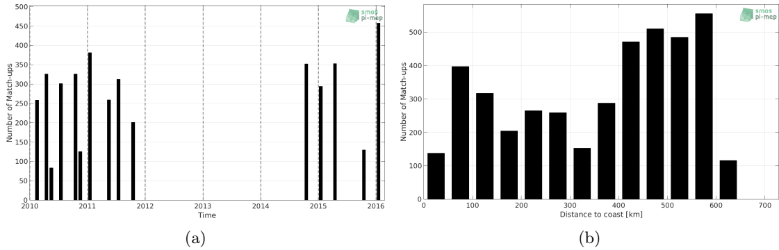
Figure 1: Number of match-ups between TSG (LEGOS-DM) and SMOS SSS L3 v4 - 9 Days (CATDS-CECOS-LOCEAN) SSS as a function of time (a) and as function of the distance to coast (b) over the Bay of Bengal Pi-MEP region and for the full satellite product period.
