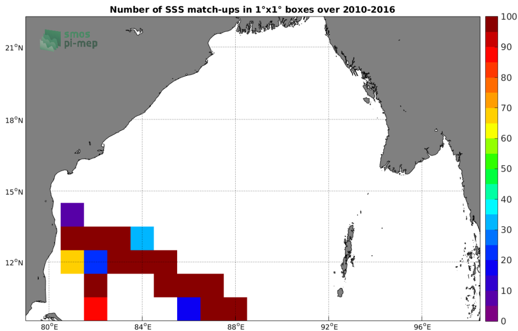
Figure 4: Number of SSS match-ups between TSG (LEGOS-DM) SSS and the SMOS SSS L3 v4 - 9 Days (CATDS-CECOS-LOCEAN) SSS product for the Bay of Bengal Pi-MEP region over 1°x1° boxes and for the full satellite product period.
