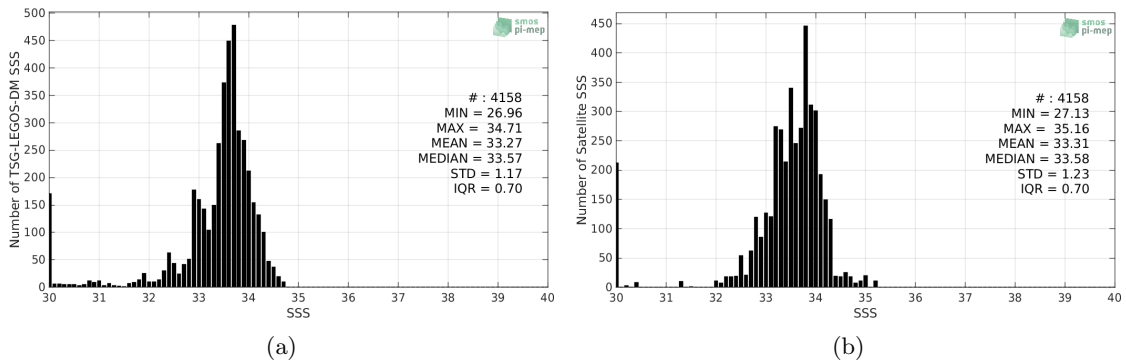
Figure 2: Histograms of SSS from TSG-LEGOS-DM (a) and SMOS-L3-CATDS-CECOS-LOCEAN-V4-9DAYS-25KM (b) considering all match-up pairs per bins of 0.1 over the Bay of Bengal Pi-MEP region and for the full satellite product period.
