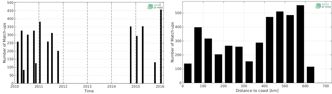
Figure 1: Number of match-ups between TSG-LEGOS-DM and SMOS-L3-CATDS-CECOS-LOCEAN-V4-9DAYS-25KM SSS as a function of time (a) and as function of the distance to coast (b) over the Bay of Bengal Pi-MEP region and for the full satellite product period.
