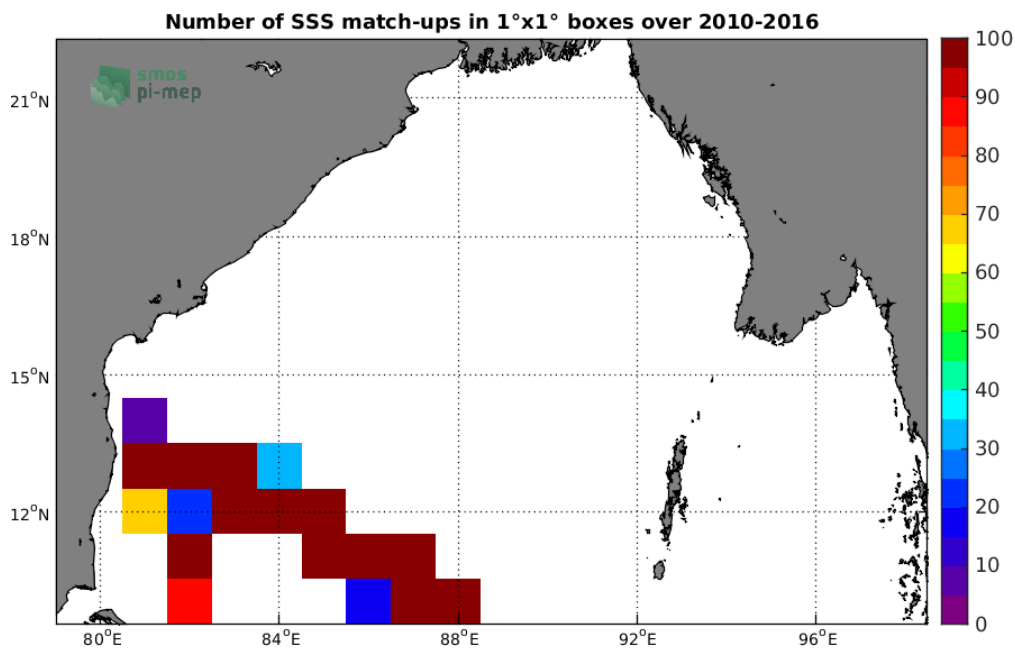
Figure 4: Number of SSS match-ups between TSG-LEGOS-DM SSS and the SMOS-L3-CATDS-CECOS-LOCEAN-V4-9DAYS-25KM SSS product for the Bay of Bengal Pi-MEP region over 1^\circ \times 1^\circ boxes and for the full satellite product period.
