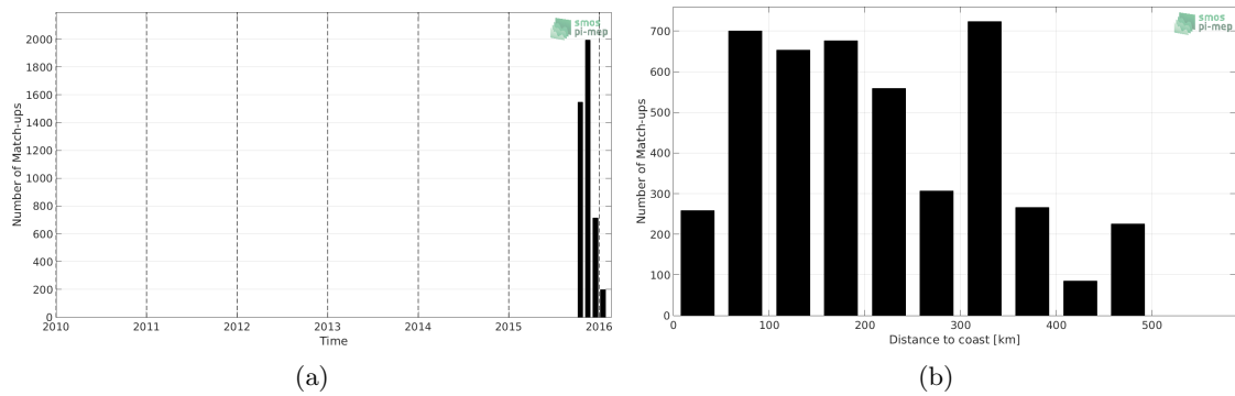
Figure 1: Number of match-ups between Surface drifters and SMOS SSS L3 v4 - 9 Days (CATDS-CECOS-LOCEAN) SSS as a function of time (a) and as function of the distance to coast (b) over the Bay of Bengal Pi-MEP region and for the full satellite product period.
