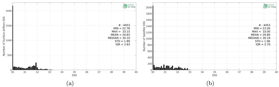
Figure 2: Histograms of SSS from Surface drifters (a) and SMOS SSS L3 v4 - 9 Days (CATDS-CECOS-LOCEAN) (b) considering all match-up pairs per bins of 0.1 over the Bay of Bengal Pi-MEP region and for the full satellite product period.
