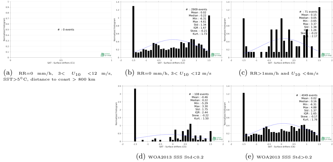
Figure 12: Normalized histogram of \Delta SSS (SMOS SSS L3 v4 - 9 Days (CATDS-CECOS-LOCEAN) - Surface drifters) for 5 different subdatasets corresponding to: RR=0 mm/h, 3 < U_{10} < 12 m/s, SST > 5°C, distance to coast > 800 km (a), RR=0 mm/h, 3 < U_{10} < 12 m/s (b), RR > 1mm/h and U_{10} < 4 m/s (c), WOA2013 SSS Std < 0.2 (d), WOA2013 SSS Std > 0.2 (e).
