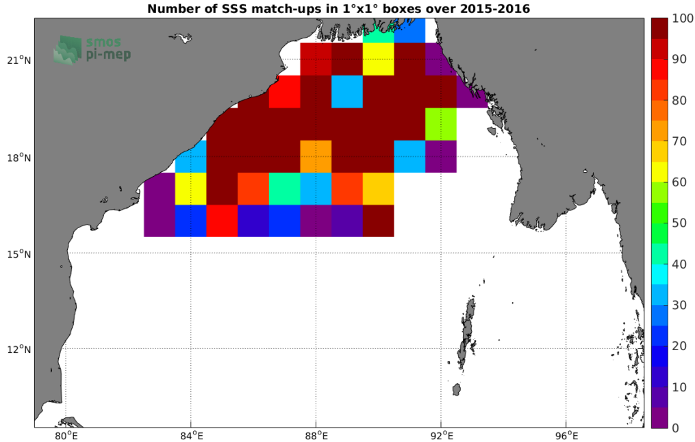
Figure 3: Number of SSS match-ups between Surface drifters SSS and the SMOS SSS L3 v4 - 9 Days (CATDS-CECOS-LOCEAN) SSS product for the Bay of Bengal Pi-MEP region over 1^\circ \times 1^\circ boxes and for the full satellite product period.
