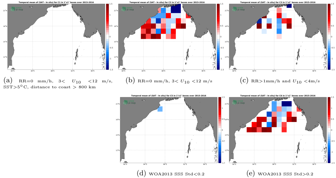
Figure 11: Temporal mean gridded over spatial boxes of size 1^{\circ}\times 1^{\circ} of \Delta\text{SSS} (SMOS SSS L3 v4 - 9 Days (CATDS-CECOS-LOCEAN) - Surface drifters) for 5 different subdatasets corresponding to:RR=0 mm/h, 3 < U_{10} < 12 m/s, SST >5^{\circ}\text{C} , distance to coast > 800 km (a), RR=0 mm/h, 3 < U_{10} < 12 m/s (b), RR >1 mm/h and U_{10} < 4 m/s (c), WOA2013 SSS Std <0.2 (d), WOA2013 SSS Std >0.2 (e).
