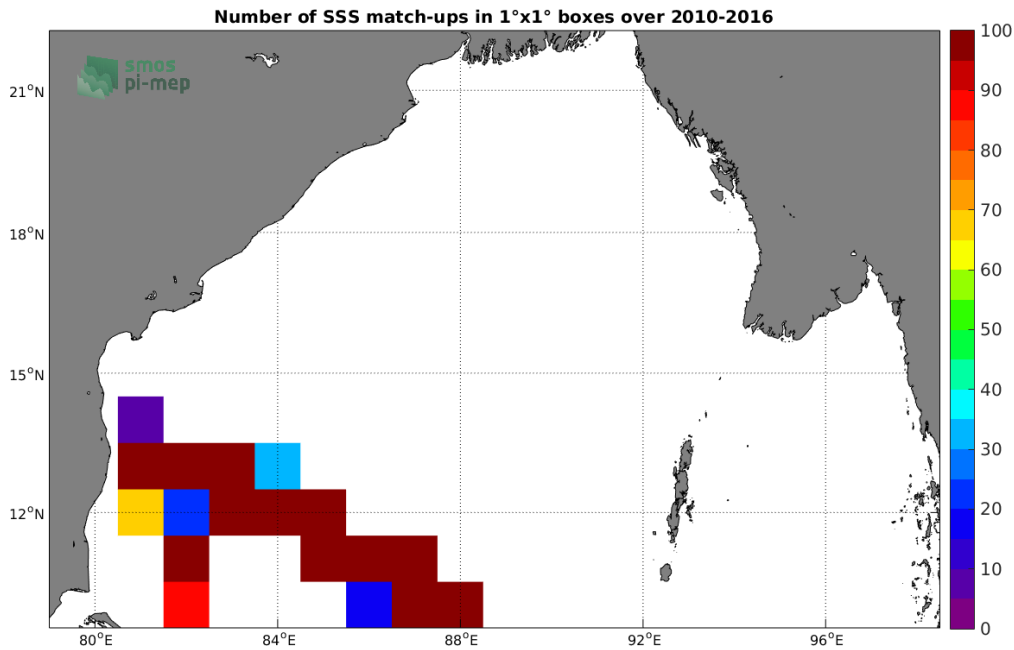
Figure 4: Number of SSS match-ups between TSG (LEGOS-DM) SSS and the SMOS SSS L3 v4 - 18 Days (CATDS-CECOS-LOCEAN) SSS product for the Bay of Bengal Pi-MEP region over 1^\circ \times 1^\circ boxes and for the full satellite product period.
