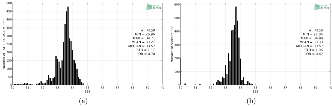
Figure 2: Histograms of SSS from TSG (LEGOS-DM) (a) and SMOS SSS L3 v4 - 18 Days (CATDS-CECOS-LOCEAN) (b) considering all match-up pairs per bins of 0.1 over the Bay of Bengal Pi-MEP region and for the full satellite product period.
