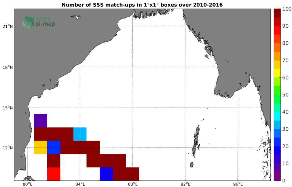
Figure 4: Number of SSS match-ups between TSG-LEGOS-DM SSS and the SMOS-L3-CATDS-CECOS-LOCEAN-V4-18DAYS-25KM SSS product for the Bay of Bengal Pi-MEP region over 1°x1° boxes and for the full satellite product period.
