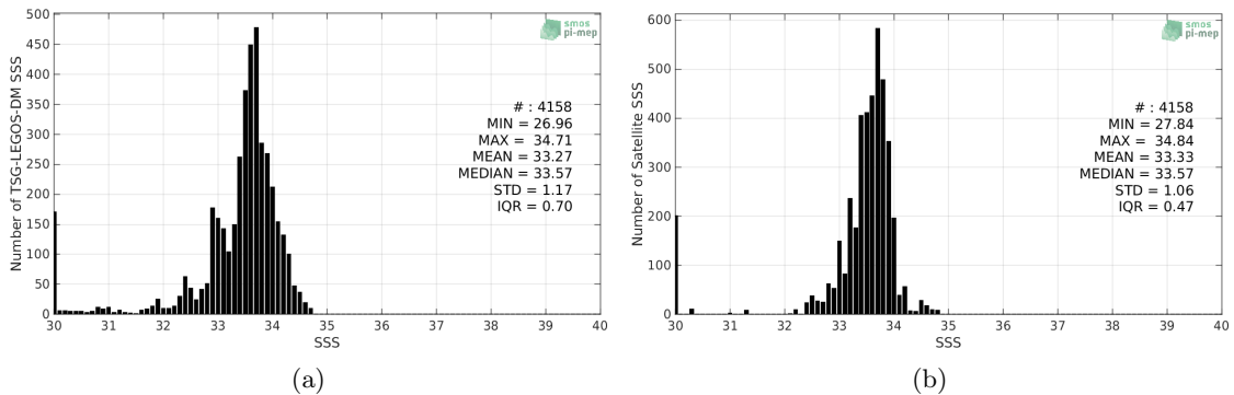
Figure 2: Histograms of SSS from TSG-LEGOS-DM (a) and SMOS-L3-CATDS-CECOS-LOCEAN-V4-18DAYS-25KM (b) considering all match-up pairs per bins of 0.1 over the Bay of Bengal Pi-MEP region and for the full satellite product period.
