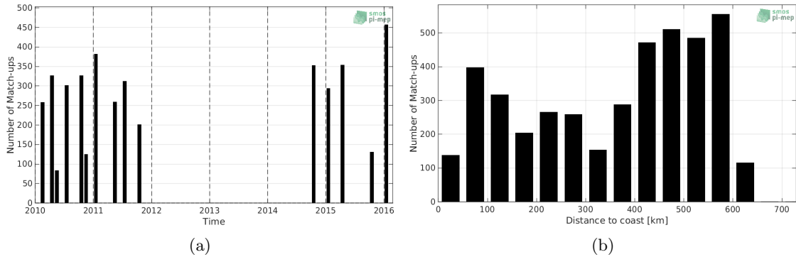
Figure 1: Number of match-ups between TSG-LEGOS-DM and SMOS-L3-CATDS-CECOS-LOCEAN-V4-18DAYS-25KM SSS as a function of time (a) and as function of the distance to coast (b) over the Bay of Bengal Pi-MEP region and for the full satellite product period.
