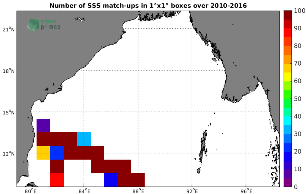
Figure 4: Number of SSS match-ups between TSG-LEGOS-DM SSS and the SMOS-L3-CATDS-CECOS-LOCEAN-V4-18DAYS-25KM SSS product for the Bay of Bengal Pi-MEP region over 1^\circ \times 1^\circ boxes and for the full satellite product period.
