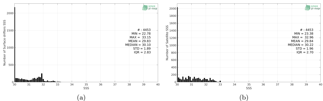
Figure 2: Histograms of SSS from Surface drifters (a) and SMOS-L3-CATDS-CECOS-LOCEAN-V4-18DAYS-25KM (b) considering all match-up pairs per bins of 0.1 over the Bay of Bengal Pi-MEP region and for the full satellite product period.
