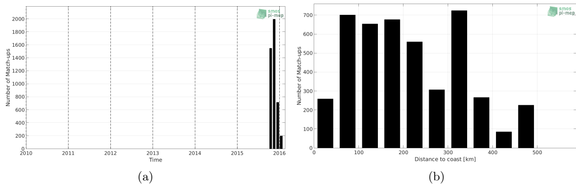
Figure 1: Number of match-ups between Surface drifters and SMOS-L3-CATDS-CECOS-LOCEAN-V4-18DAYS-25KM SSS as a function of time (a) and as function of the distance to coast (b) over the Bay of Bengal Pi-MEP region and for the full satellite product period.
