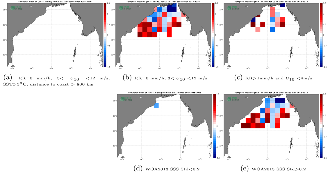
Figure 11: Temporal mean gridded over spatial boxes of size 1^{\circ}\times 1^{\circ} of \Delta\text{SSS} (SMOS-L3-CATDS-CECOS-LOCEAN-V4-18DAYS-25KM - Surface drifters) for 5 different subdatasets corresponding to:RR=0 mm/h, 3 < U_{10} < 12 m/s, SST >5^{\circ}\text{C} , distance to coast > 800 km (a), RR=0 mm/h, 3 < U_{10} < 12 m/s (b), RR >1 mm/h and U_{10} < 4 m/s (c), WOA2013 SSS Std <0.2 (d), WOA2013 SSS Std >0.2 (e).
