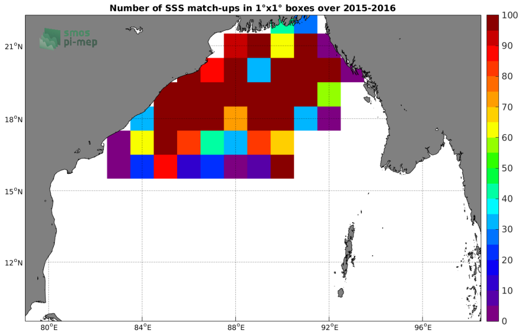
Figure 3: Number of SSS match-ups between Surface drifters SSS and the SMOS-L3-CATDS-CECOS-LOCEAN-V4-18DAYS-25KM SSS product for the Bay of Bengal Pi-MEP region over 1°x1° boxes and for the full satellite product period.
