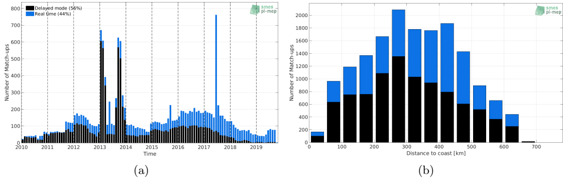
Figure 1: Number of match-ups between Argo and SMOS SSS L3 v4 - 18 Days (CATDS-CECOS-LOCEAN) SSS as a function of time (a) and as function of the distance to coast (b) over the Bay of Bengal Pi-MEP region and for the full satellite product period.
