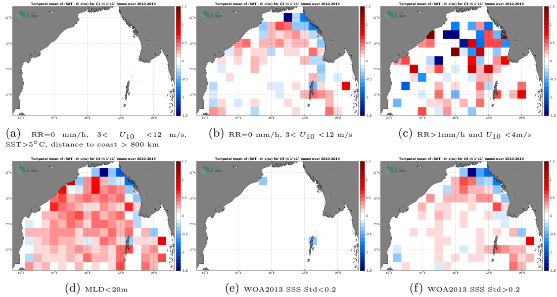
Figure 12: Temporal mean gridded over spatial boxes of size 1^\circ \times 1^\circ of \Delta SSS (SMOS SSS L3 v4 - 18 Days (CATDS-CECOS-LOCEAN) - Argo) for 6 different subdatasets corresponding to: RR=0 mm/h, 3 < U_{10} < 12 m/s, SST > 5^\circ C , distance to coast > 800 km (a), RR=0 mm/h, 3 < U_{10} < 12 m/s (b), RR > 1 mm/h and U_{10} < 4 m/s (c), MLD < 20 m (d), WOA2013 SSS Std < 0.2 (e), WOA2013 SSS Std > 0.2 (f).
