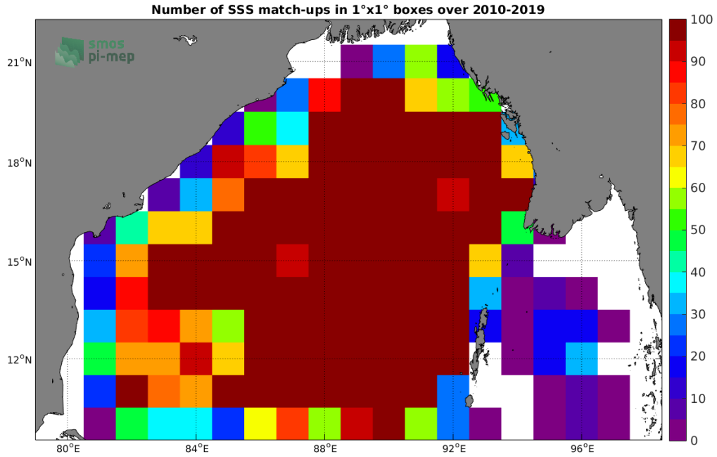
Figure 4: Number of SSS match-ups between Argo SSS and the SMOS SSS L3 v4 - 18 Days (CATDS-CECOS-LOCEAN) SSS product for the Bay of Bengal Pi-MEP region over 1°x1° boxes and for the full satellite product period.
