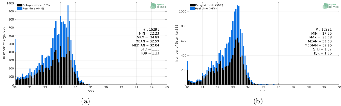
Figure 2: Histograms of SSS from Argo (a) and SMOS SSS L3 v4 - 18 Days (CATDS-CECOS-LOCEAN) (b) considering all match-up pairs per bins of 0.1 over the Bay of Bengal Pi-MEP region and for the full satellite product period.
