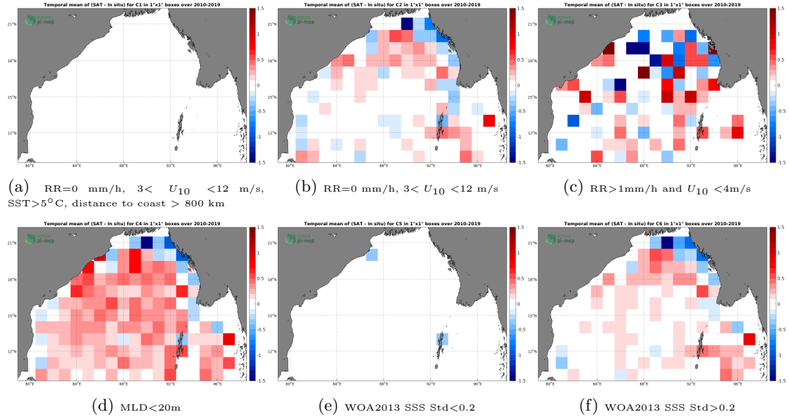
Figure 12: Temporal mean gridded over spatial boxes of size 1^\circ \times 1^\circ of \Delta SSS (SMOS-L3-CATDS-CECOS-LOCEAN-V4-18DAYS-25KM - Argo) for 6 different subdatasets corresponding to:RR=0 mm/h, 3 < U_{10} < 12 m/s, SST >5^\circ\text{C} , distance to coast > 800 km (a), RR=0 mm/h, 3 < U_{10} < 12 m/s (b), RR >1 mm/h and U_{10} < 4 m/s (c),MLD <20 m (d),WOA2013 SSS Std <0.2 (e),WOA2013 SSS Std >0.2 (f).
