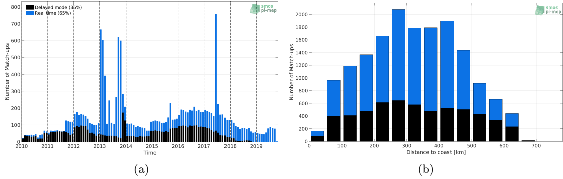
Figure 1: Number of match-ups between Argo and SMOS-L3-CATDS-CECOS-LOCEAN-V4-18DAYS-25KM SSS as a function of time (a) and as function of the distance to coast (b) over the Bay of Bengal Pi-MEP region and for the full satellite product period.
