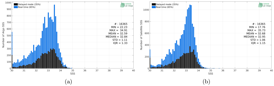
Figure 2: Histograms of SSS from Argo (a) and SMOS-L3-CATDS-CECOS-LOCEAN-V4-18DAYS-25KM (b) considering all match-up pairs per bins of 0.1 over the Bay of Bengal Pi-MEP region and for the full satellite product period.
