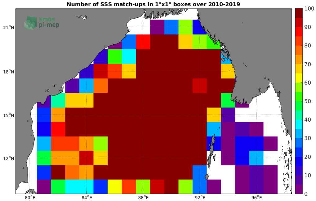
Figure 4: Number of SSS match-ups between Argo SSS and the SMOS-L3-CATDS-CECOS-LOCEAN-V4-18DAYS-25KM SSS product for the Bay of Bengal Pi-MEP region over 1°x1° boxes and for the full satellite product period.
