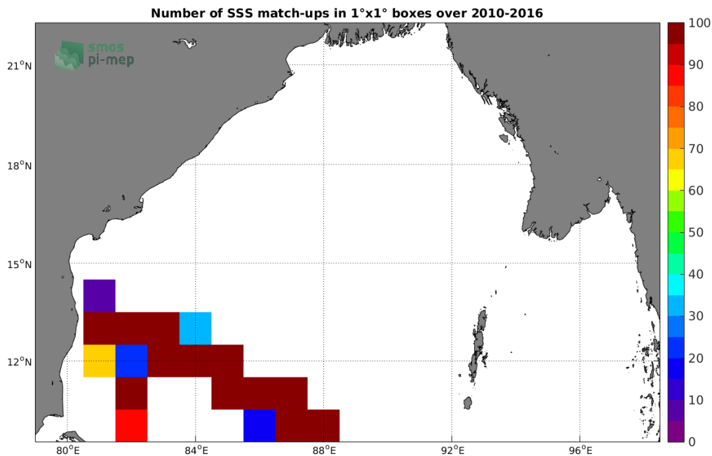
Figure 4: Number of SSS match-ups between TSG-LEGOS-DM SSS and the SMOS-L3-CATDS-CECOS-LOCEAN-V3-18DAYS-25KM SSS product for the Bay of Bengal Pi-MEP region over 1°x1° boxes and for the full satellite product period.
