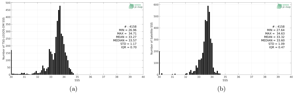
Figure 2: Histograms of SSS from TSG-LEGOS-DM (a) and SMOS-L3-CATDS-CECOS-LOCEAN-V3-18DAYS-25KM (b) considering all match-up pairs per bins of 0.1 over the Bay of Bengal Pi-MEP region and for the full satellite product period.
