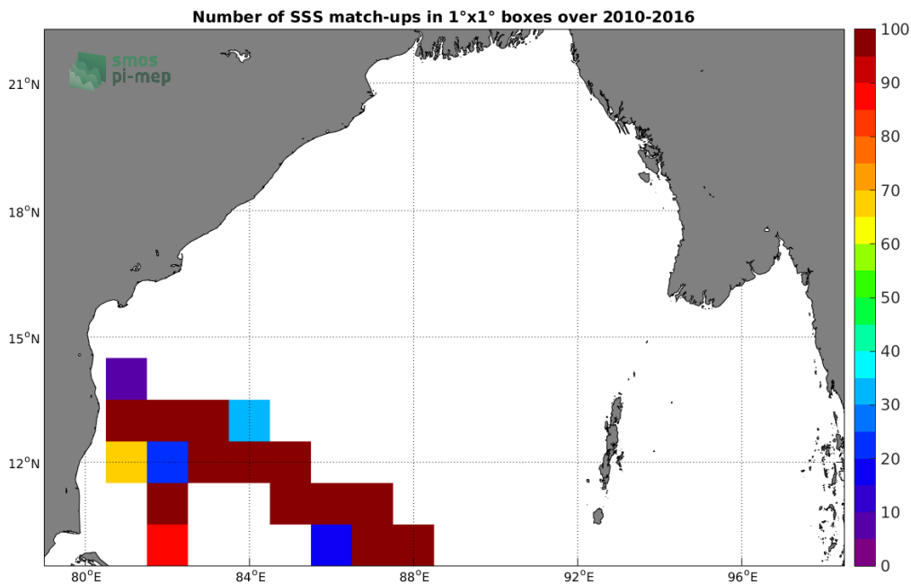
Figure 4: Number of SSS match-ups between TSG-LEGOS-DM SSS and the SMOS-L3-CATDS-CECOS-LOCEAN-V3-18DAYS-25KM SSS product for the Bay of Bengal Pi-MEP region over 1^\circ \times 1^\circ boxes and for the full satellite product period.
