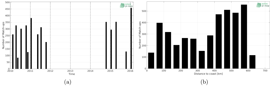
Figure 1: Number of match-ups between TSG-LEGOS-DM and SMOS-L3-CATDS-CECOS-LOCEAN-V3-18DAYS-25KM SSS as a function of time (a) and as function of the distance to coast (b) over the Bay of Bengal Pi-MEP region and for the full satellite product period.
