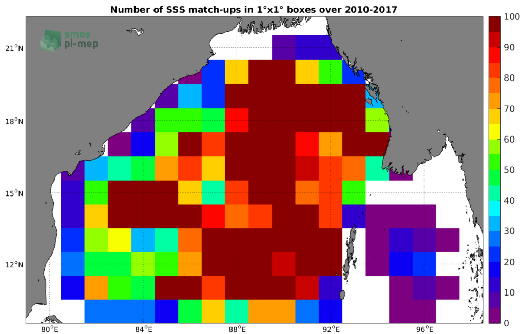
Figure 4: Number of SSS match-ups between Argo SSS and the SMOS-L3-CATDS-CECOS-LOCEAN-V3-18DAYS-25KM SSS product for the Bay of Bengal Pi-MEP region over 1^{\circ} \times 1^{\circ} boxes and for the full satellite product period.
