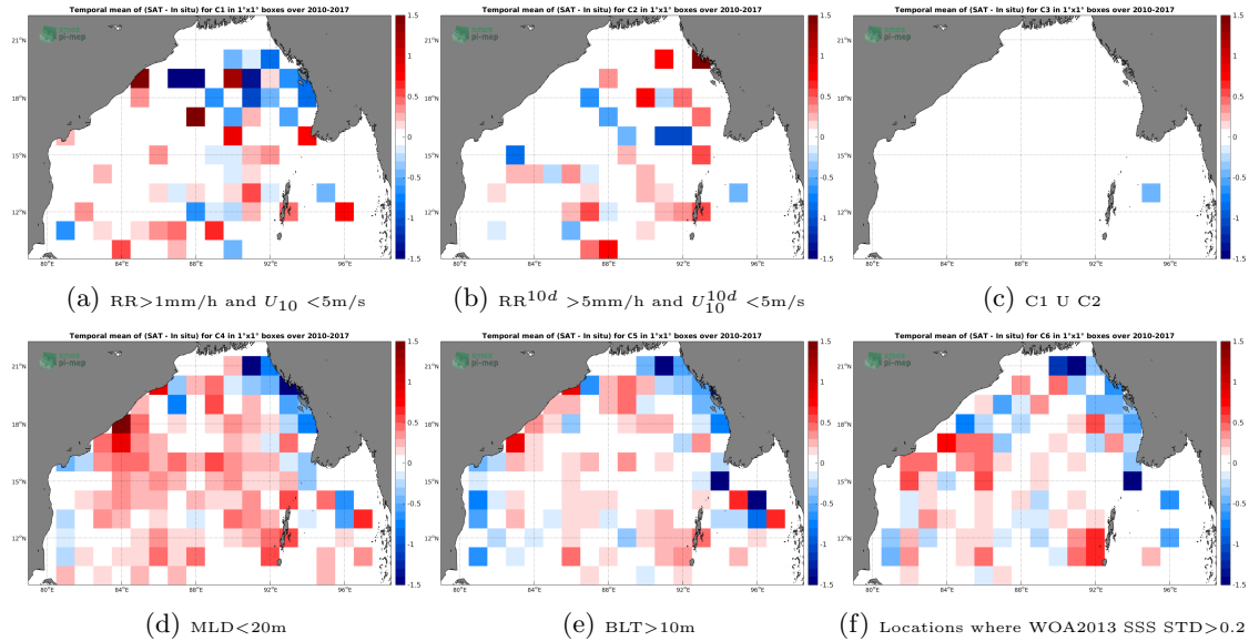
Figure 12: Temporal mean gridded over spatial boxes of size 1^\circ \times 1^\circ of \Delta\text{SSS} (SMOS-L3-CATDS-CECOS-LOCEAN-V3-18DAYS-25KM - Argo) for 6 different subdatasets corresponding to: \text{RR} > 1\text{mm/h} and U_{10} < 5\text{m/s} (a), \text{RR}^{10d} > 5\text{mm/h} and U_{10}^{10d} < 5\text{m/s} (b), C1 U C2 (c), \text{MLD} < 20\text{m} (d), \text{BLT} > 10\text{m} (e), Locations where WOA2013 SSS STD > 0.2 (f).
