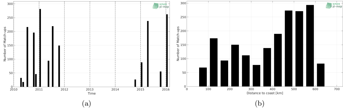
Figure 1: Number of match-ups between TSG (LEGOS-DM) and SMOS SSS L3 v2 - Monthly - 0.25 Deg (CATDS-CECOS-IFREMER) SSS as a function of time (a) and as function of the distance to coast (b) over the Bay of Bengal Pi-MEP region and for the full satellite product period.
