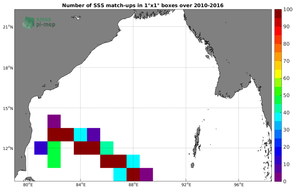
Figure 4: Number of SSS match-ups between TSG (LEGOS-DM) SSS and the SMOS SSS L3 v2 - Monthly - 0.25 Deg (CATDS-CECOS-IFREMER) SSS product for the Bay of Bengal Pi-MEP region over 1°x1° boxes and for the full satellite product period.
