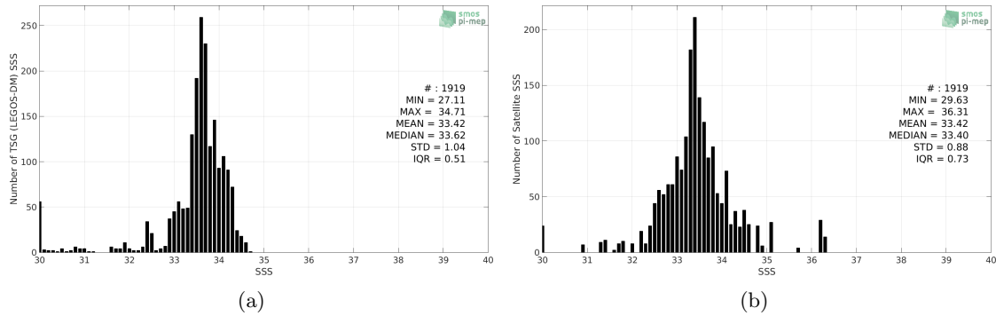
Figure 2: Histograms of SSS from TSG (LEGOS-DM) (a) and SMOS SSS L3 v2 - Monthly - 0.25 Deg (CATDS-CECOS-IFREMER) (b) considering all match-up pairs per bins of 0.1 over the Bay of Bengal Pi-MEP region and for the full satellite product period.
