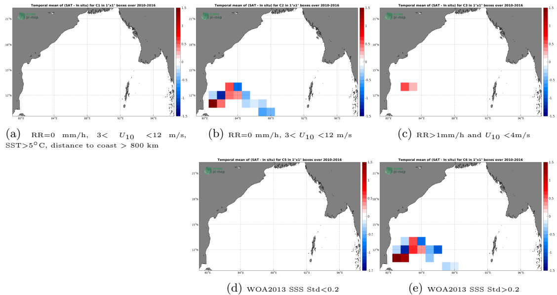
Figure 12: Temporal mean gridded over spatial boxes of size 1^{\circ}\times 1^{\circ} of \Delta\text{SSS} (SMOS L3 v2 - Monthly - 0.25 Deg (CATDS-CECOS-IFREMER) - TSG-LEGOS-DM) for 5 different subdatasets corresponding to: RR=0 mm/h, 3 < U_{10} < 12 m/s, SST > 5^{\circ}\text{C} , distance to coast > 800 km (a), RR=0 mm/h, 3 < U_{10} < 12 m/s (b), RR > 1 mm/h and U_{10} < 4 m/s (c), WOA2013 SSS Std < 0.2 (d), WOA2013 SSS Std > 0.2 (e).
