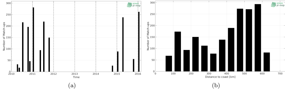
Figure 1: Number of match-ups between TSG-LEGOS-DM and SMOS L3 v2 - Monthly - 0.25 Deg (CATDS-CECOS-IFREMER) SSS as a function of time (a) and as function of the distance to coast (b) over the Bay of Bengal Pi-MEP region and for the full satellite product period.
