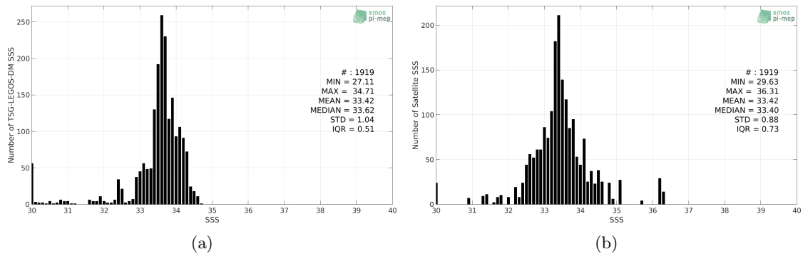
Figure 2: Histograms of SSS from TSG-LEGOS-DM (a) and SMOS L3 v2 - Monthly - 0.25 Deg (CATDS-CECOS-IFREMER) (b) considering all match-up pairs per bins of 0.1 over the Bay of Bengal Pi-MEP region and for the full satellite product period.
