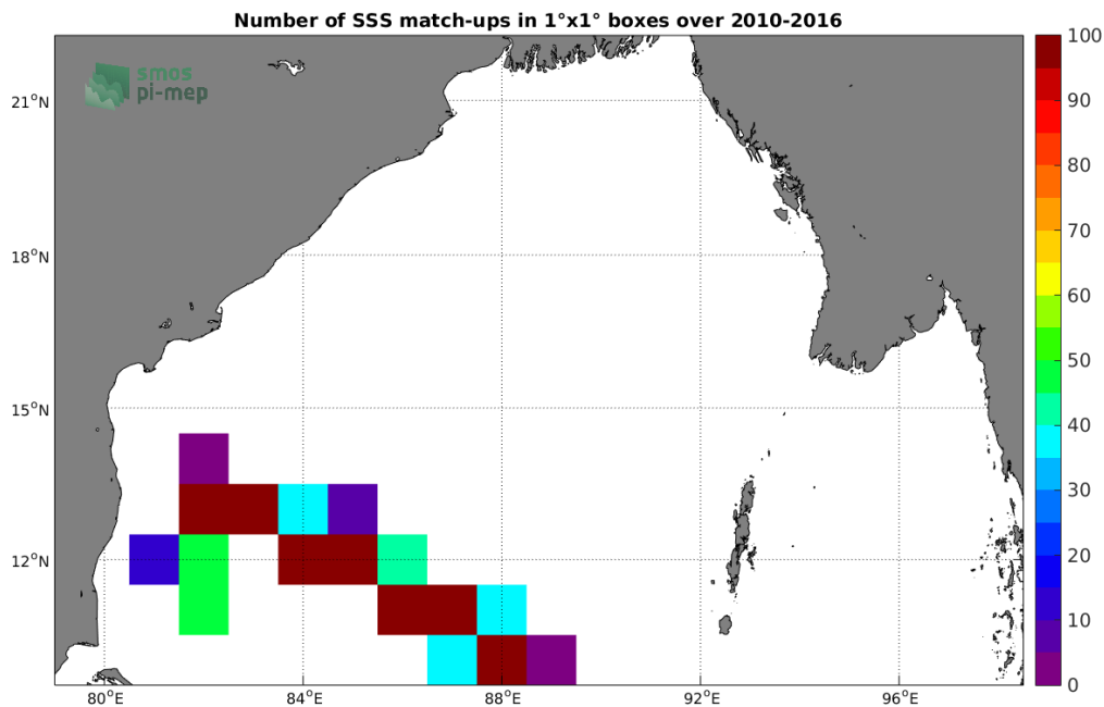
Figure 4: Number of SSS match-ups between TSG-LEGOS-DM SSS and the SMOS L3 v2 - Monthly - 0.25 Deg (CATDS-CECOS-IFREMER) SSS product for the Bay of Bengal Pi-MEP region over 1^\circ \times 1^\circ boxes and for the full satellite product period.
