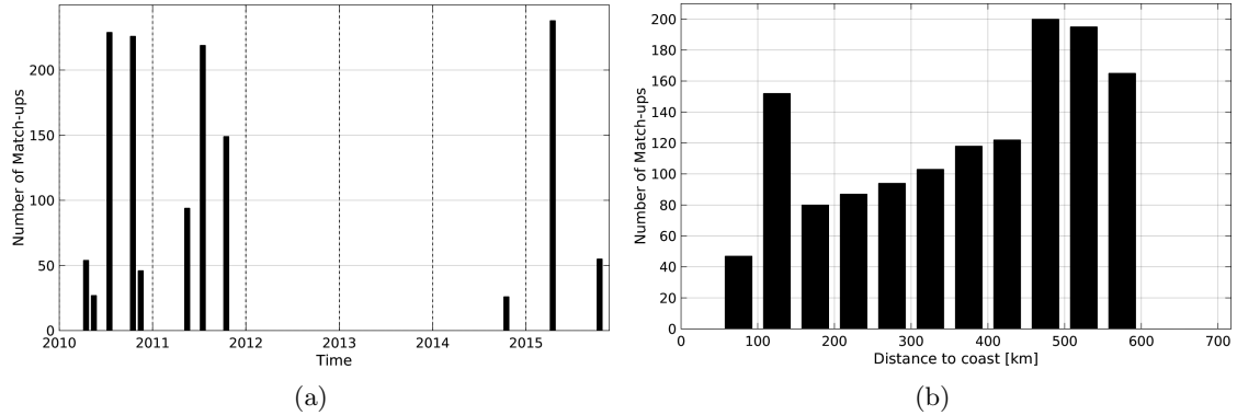
Figure 1: Number of match-ups between TSG-LEGOS-DM and SMOS-L3-CATDS-IFREMER-CECOS-V2-MONTHLY-0.25DEG SSS as a function of time (a) and as function of the distance to coast (b) over the Bay of Bengal Pi-MEP region and for the full satellite product period.
