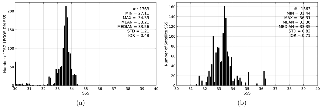
Figure 2: Histograms of SSS from TSG-LEGOS-DM (a) and SMOS-L3-CATDS-IFREMER-CECOS-V2-MONTHLY-0.25DEG (b) considering all match-up pairs per bins of 0.1 over the Bay of Bengal Pi-MEP region and for the full satellite product period.
