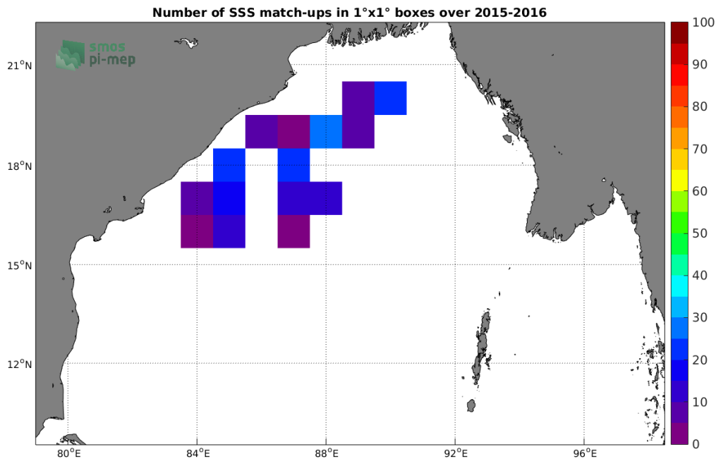
Figure 3: Number of SSS match-ups between Surface drifters SSS and the SMOS L3 v2 - Monthly - 0.25 Deg (CATDS-CECOS-IFREMER) SSS product for the Bay of Bengal Pi-MEP region over 1°x1° boxes and for the full satellite product period.
