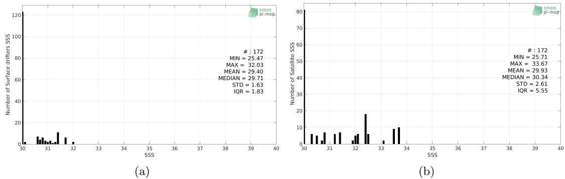
Figure 2: Histograms of SSS from Surface drifters (a) and SMOS L3 v2 - Monthly - 0.25 Deg (CATDS-CECOS-IFREMER) (b) considering all match-up pairs per bins of 0.1 over the Bay of Bengal Pi-MEP region and for the full satellite product period.
