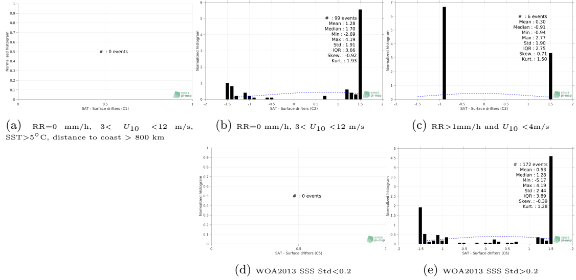
Figure 12: Normalized histogram of \Delta\text{SSS} (SMOS L3 v2 - Monthly - 0.25 Deg (CATDS-CECOS-IFREMER) - Surface drifters) for 5 different subdatasets corresponding to: RR=0 mm/h, 3 < U_{10} < 12 m/s, SST > 5^{\circ}\text{C} , distance to coast > 800 km (a), RR=0 mm/h, 3 < U_{10} < 12 m/s (b), RR > 1\text{mm/h} and U_{10} < 4\text{m/s} (c), WOA2013 SSS Std < 0.2 (d), WOA2013 SSS Std > 0.2 (e).
