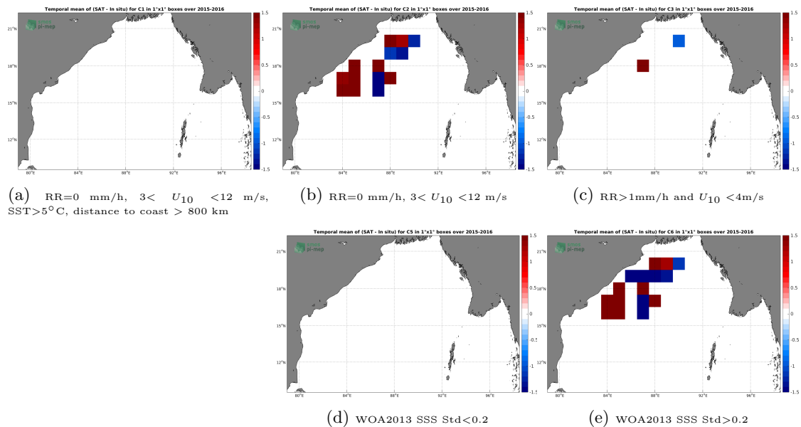
Figure 11: Temporal mean gridded over spatial boxes of size 1^{\circ}\times 1^{\circ} of \Delta\text{SSS} (SMOS L3 v2 - Monthly - 0.25 Deg (CATDS-CECOS-IFREMER) - Surface drifters) for 5 different subdatasets corresponding to:RR=0 mm/h, 3 < U_{10} < 12 m/s, SST >5^{\circ}\text{C} , distance to coast > 800 km (a), RR=0 mm/h, 3 < U_{10} < 12 m/s (b), RR >1 mm/h and U_{10} < 4 m/s (c), WOA2013 SSS Std <0.2 (d), WOA2013 SSS Std >0.2 (e).
