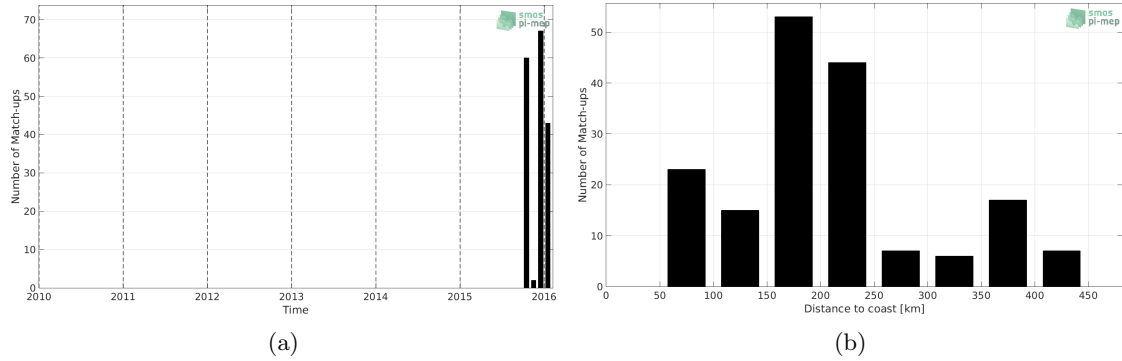
Figure 1: Number of match-ups between Surface drifters and SMOS L3 v2 - Monthly - 0.25 Deg (CATDS-CECOS-IFREMER) SSS as a function of time (a) and as function of the distance to coast (b) over the Bay of Bengal Pi-MEP region and for the full satellite product period.
