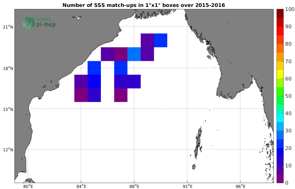
Figure 3: Number of SSS match-ups between Surface drifters SSS and the SMOS-L3-CATDS-IFREMER-CECOS-V2-MONTHLY-0.25DEG SSS product for the Bay of Bengal Pi-MEP region over 1°x1° boxes and for the full satellite product period.
