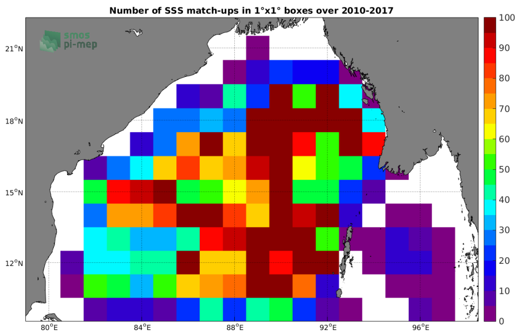
Figure 4: Number of SSS match-ups between Argos SSS and the SMOS-L3-CATDS-IFREMER-CECOS-V2-MONTHLY-0.25DEG SSS product for the Bay of Bengal Pi-MEP region over 1^\circ \times 1^\circ boxes and for the full satellite product period.
