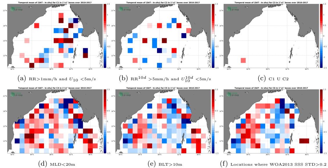
Figure 12: Temporal mean gridded over spatial boxes of size 1^\circ \times 1^\circ of \Delta\text{SSS} (SMOS-L3-CATDS-IFREMER-CECOS-V2-MONTHLY-0.25DEG - Argo) for 6 different subdatasets corresponding to: \text{RR} > 1\text{mm/h} and U_{10} < 5\text{m/s} (a), \text{RR}^{10d} > 5\text{mm/h} and U_{10}^{10d} < 5\text{m/s} (b), C1 U C2 (c), \text{MLD} < 20\text{m} (d), \text{BLT} > 10\text{m} (e), Locations where WOA2013 SSS STD > 0.2 (f).
