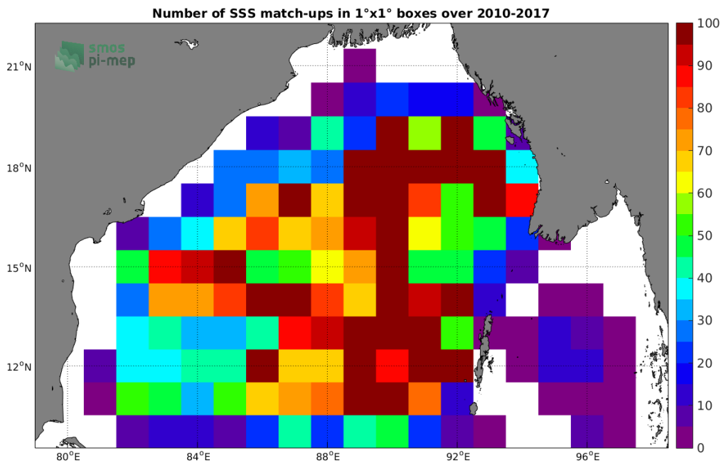
Figure 4: Number of SSS match-ups between Argos SSS and the SMOS-L3-CATDS-IFREMER-CECOS-V2-MONTHLY-0.25DEG SSS product for the Bay of Bengal Pi-MEP region over 1^{\circ} \times 1^{\circ} boxes and for the full satellite product period.
