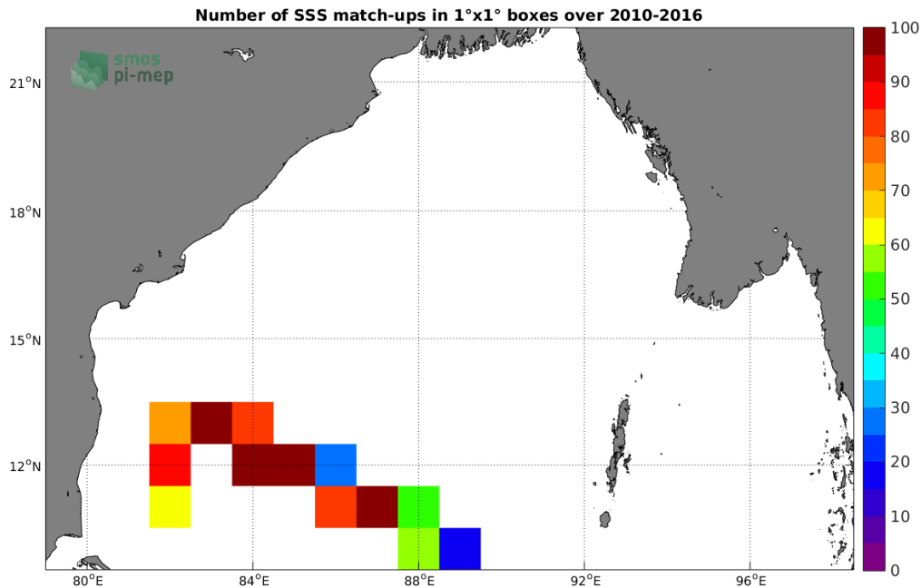
Figure 4: Number of SSS match-ups between TSG (LEGOS-DM) SSS and the SMOS SSS L3 v2 - Daily - 0.5 Deg (CATDS-CECOS-IFREMER) SSS product for the Bay of Bengal Pi-MEP region over 1°x1° boxes and for the full satellite product period.
