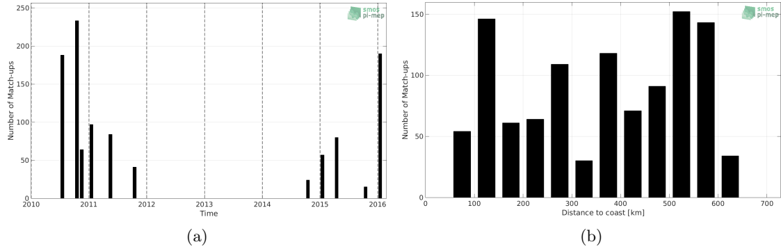
Figure 1: Number of match-ups between TSG-LEGOS-DM and SMOS L3 v2 - Daily - 0.5 Deg (CATDS-CECOS-IFREMER) SSS as a function of time (a) and as function of the distance to coast (b) over the Bay of Bengal Pi-MEP region and for the full satellite product period.
