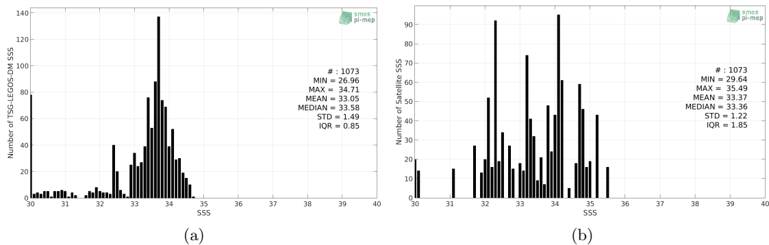
Figure 2: Histograms of SSS from TSG-LEGOS-DM (a) and SMOS L3 v2 - Daily - 0.5 Deg (CATDS-CECOS-IFREMER) (b) considering all match-up pairs per bins of 0.1 over the Bay of Bengal Pi-MEP region and for the full satellite product period.
