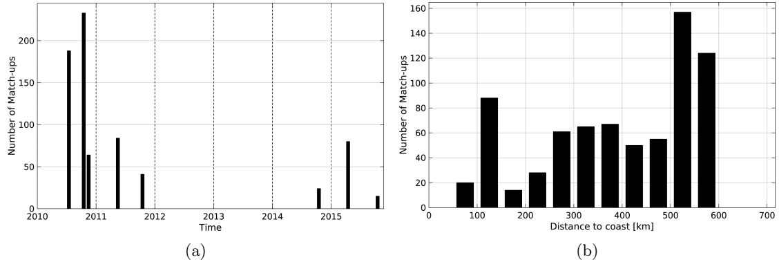
Figure 1: Number of match-ups between TSG-LEGOS-DM and SMOS-L3-CATDS-CECOS-IFREMER-V2-1DAY-0.5DEG SSS as a function of time (a) and as function of the distance to coast (b) over the Bay of Bengal Pi-MEP region and for the full satellite product period.
