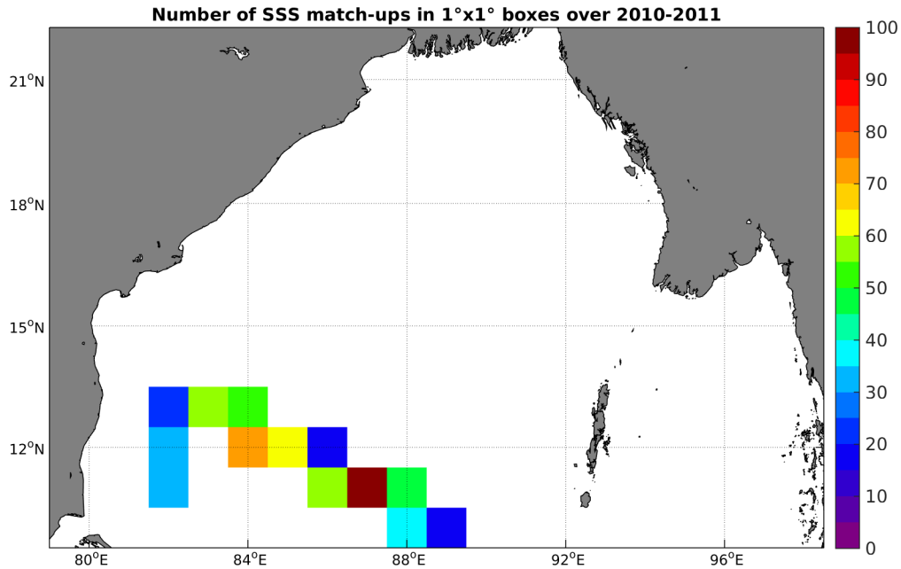
Figure 4: Number of SSS match-ups between TSG-LEGOS-DM SSS and the SMOS-L3-CATDS-CECOS-IFREMER-V2-1DAY-0.5deg SSS product for the Bay of Bengal Pi-MEP region over 1^{\circ} \times 1^{\circ} boxes and for the full satellite product period.
