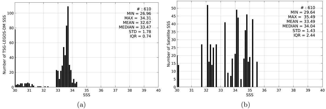
Figure 2: Histograms of SSS from TSG-LEGOS-DM (a) and SMOS-L3-CATDS-CECOS-IFREMER-V2-1DAY-0.5deg (b) considering all match-up pairs per bins of 0.1 over the Bay of Bengal Pi-MEP region and for the full satellite product period.
