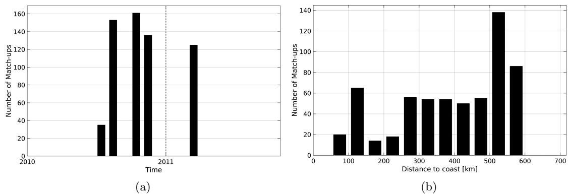
Figure 1: Number of match-ups between TSG-LEGOS-DM and SMOS-L3-CATDS-CECOS-IFREMER-V2-1DAY-0.5deg SSS as a function of time (a) and as function of the distance to coast (b) over the Bay of Bengal Pi-MEP region and for the full satellite product period.
