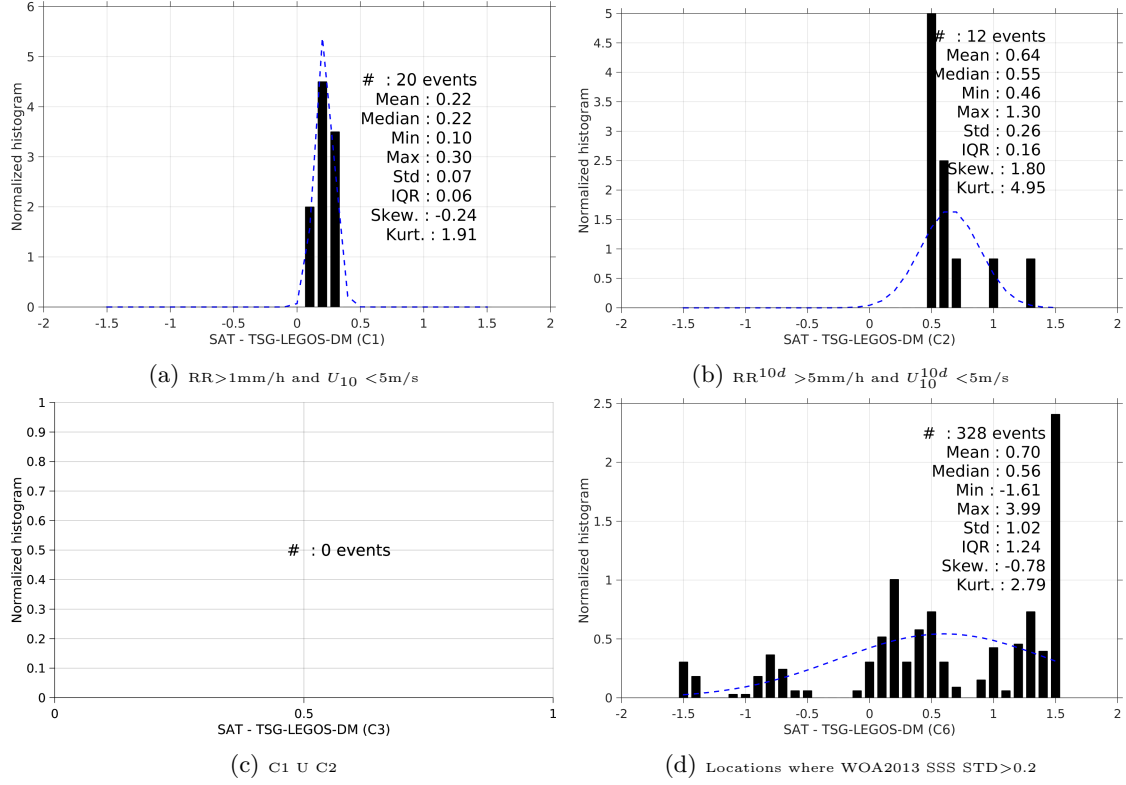
Figure 13: Normalized histogram of \Delta\text{SSS} (SMOS-L3-CATDS-CECOS-IFREMER-V2-1DAY-0.5deg - TSG-LEGOS-DM) for 6 different subdatasets corresponding to: RR > 1mm/h and U_{10} < 5\text{m/s} (a), RR^{10d} > 5\text{mm/h} and U_{10}^{10d} < 5\text{m/s} (b), C1 U C2 (c), Locations where WOA2013 SSS STD > 0.2 (d).
