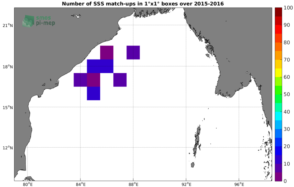
Figure 3: Number of SSS match-ups between Surface drifters SSS and the SMOS SSS L3 v2 - Daily - 0.5 Deg (CATDS-CECOS-IFREMER) SSS product for the Bay of Bengal Pi-MEP region over 1°x1° boxes and for the full satellite product period.
