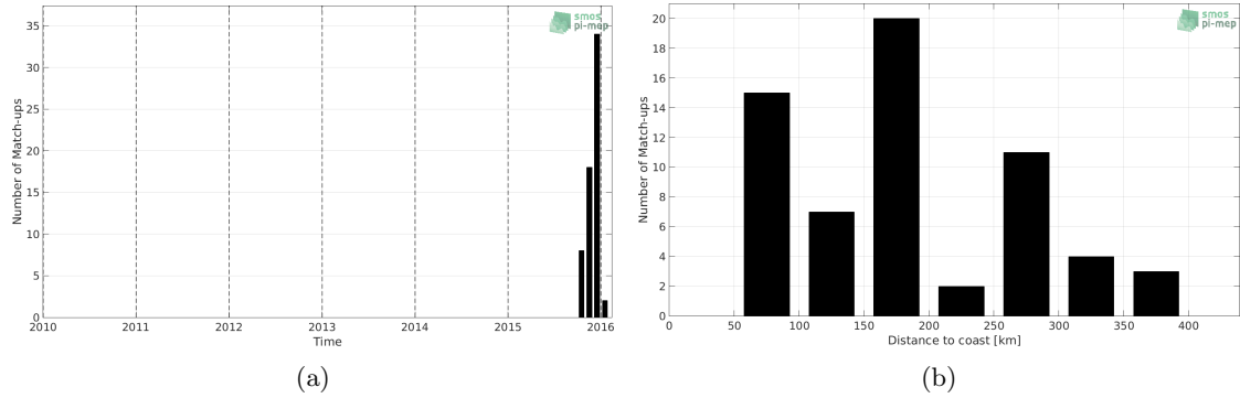
Figure 1: Number of match-ups between Surface drifters and SMOS SSS L3 v2 - Daily - 0.5 Deg (CATDS-CECOS-IFREMER) SSS as a function of time (a) and as function of the distance to coast (b) over the Bay of Bengal Pi-MEP region and for the full satellite product period.
