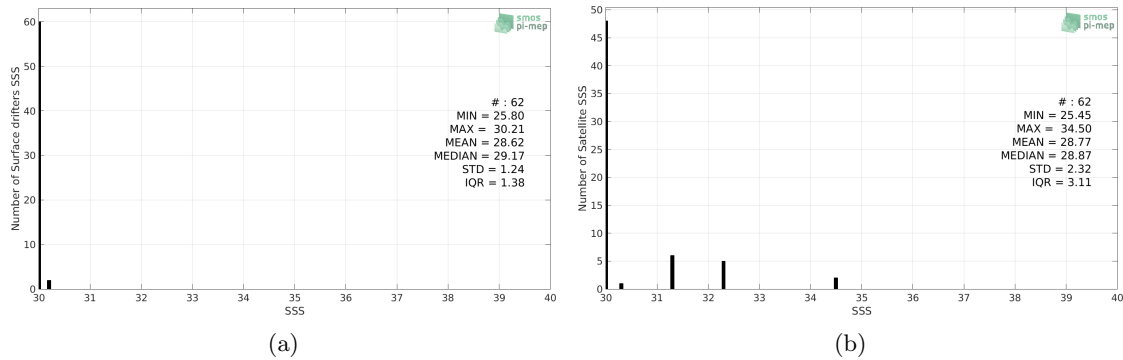
Figure 2: Histograms of SSS from Surface drifters (a) and SMOS SSS L3 v2 - Daily - 0.5 Deg (CATDS-CECOS-IFREMER) (b) considering all match-up pairs per bins of 0.1 over the Bay of Bengal Pi-MEP region and for the full satellite product period.
