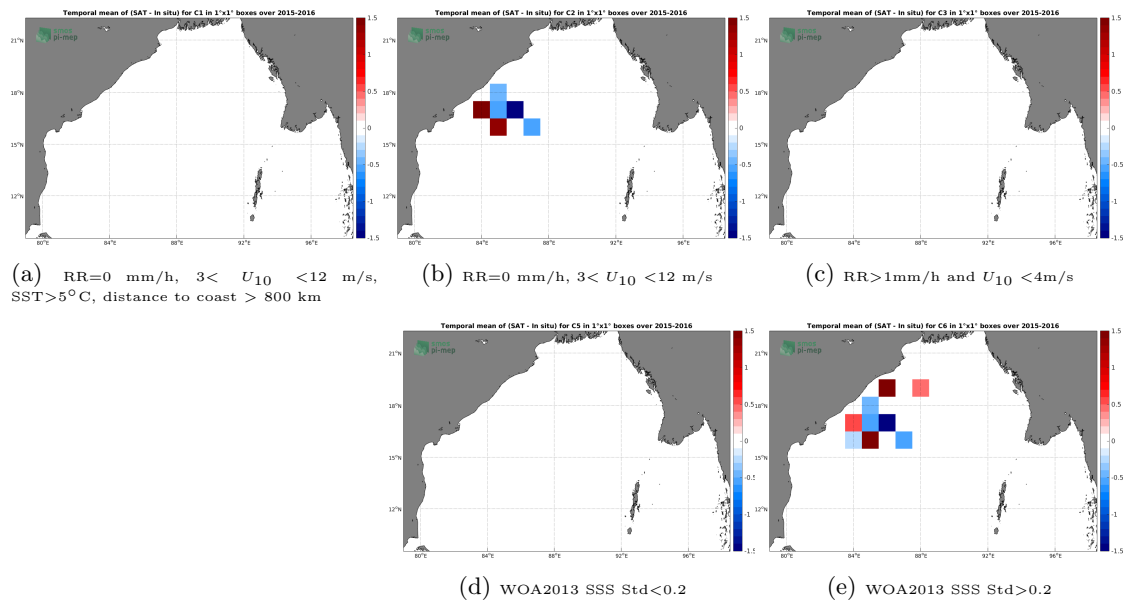
Figure 11: Temporal mean gridded over spatial boxes of size 1^{\circ}\times 1^{\circ} of \Delta\text{SSS} (SMOS L3 v2 - Daily - 0.5 Deg (CATDS-CECOS-IFREMER) - Surface drifters) for 5 different subdatasets corresponding to:RR=0 mm/h, 3 < U_{10} < 12 m/s, SST >5^{\circ}\text{C} , distance to coast > 800 km (a), RR=0 mm/h, 3 < U_{10} < 12 m/s (b), RR >1 mm/h and U_{10} < 4 m/s (c), WOA2013 SSS Std <0.2 (d), WOA2013 SSS Std >0.2 (e).
