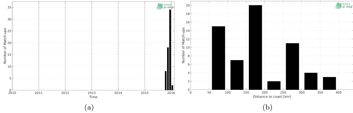
Figure 1: Number of match-ups between Surface drifters and SMOS L3 v2 - Daily - 0.5 Deg (CATDS-CECOS-IFREMER) SSS as a function of time (a) and as function of the distance to coast (b) over the Bay of Bengal Pi-MEP region and for the full satellite product period.
