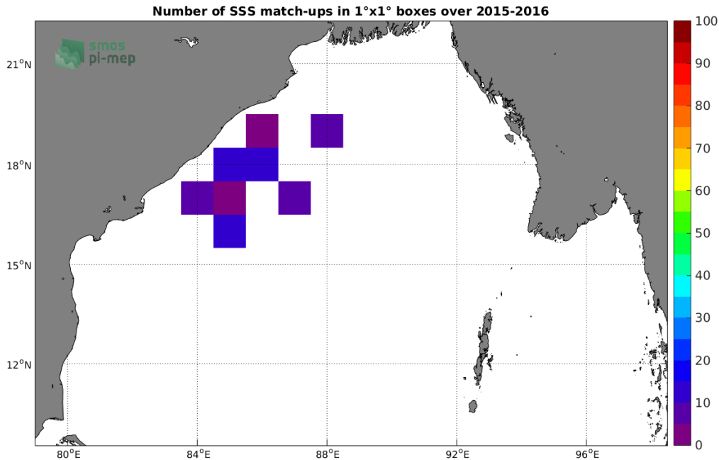
Figure 3: Number of SSS match-ups between Surface drifters SSS and the SMOS L3 v2 - Daily - 0.5 Deg (CATDS-CECOS-IFREMER) SSS product for the Bay of Bengal Pi-MEP region over 1°x1° boxes and for the full satellite product period.
