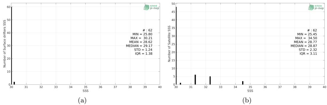
Figure 2: Histograms of SSS from Surface drifters (a) and SMOS L3 v2 - Daily - 0.5 Deg (CATDS-CECOS-IFREMER) (b) considering all match-up pairs per bins of 0.1 over the Bay of Bengal Pi-MEP region and for the full satellite product period.
