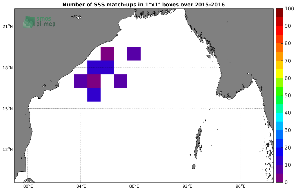
Figure 3: Number of SSS match-ups between Surface drifters SSS and the SMOS-L3-CATDS-CECOS-IFREMER-V2-1DAY-0.5DEG SSS product for the Bay of Bengal Pi-MEP region over 1°x1° boxes and for the full satellite product period.
