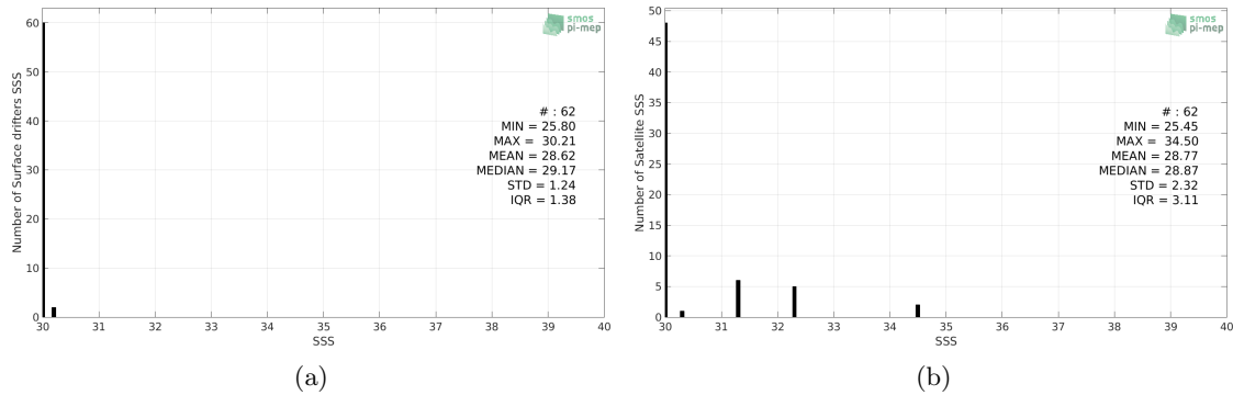
Figure 2: Histograms of SSS from Surface drifters (a) and SMOS-L3-CATDS-CECOS-IFREMER-V2-1DAY-0.5DEG (b) considering all match-up pairs per bins of 0.1 over the Bay of Bengal Pi-MEP region and for the full satellite product period.
