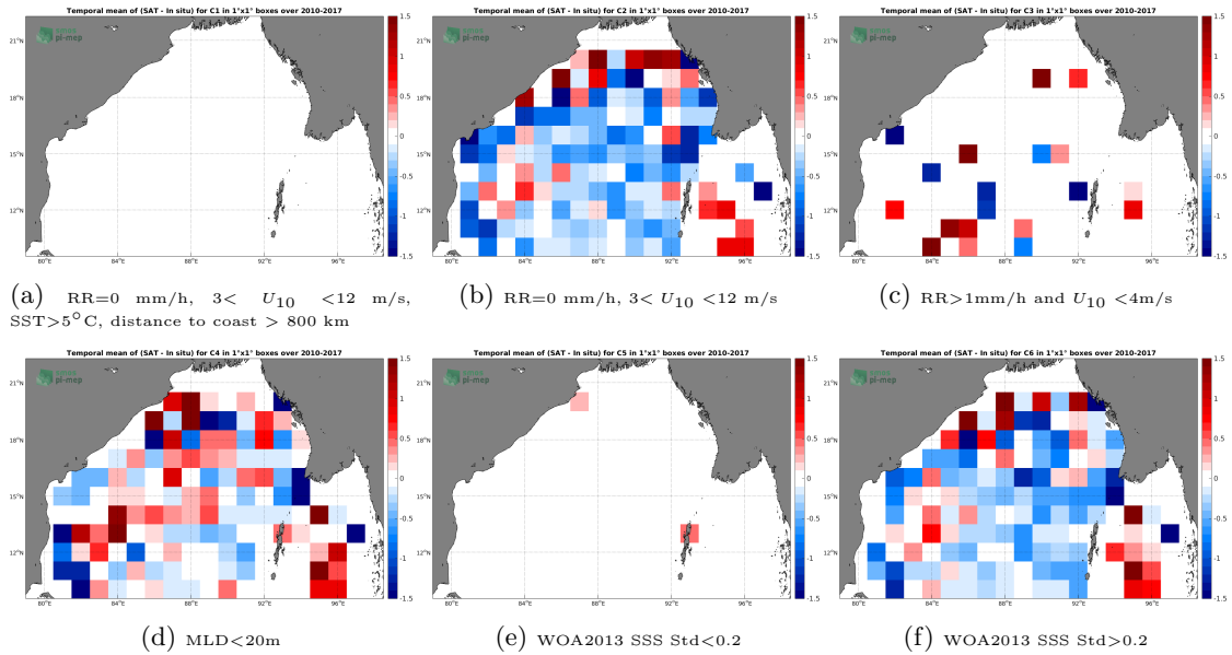
Figure 12: Temporal mean gridded over spatial boxes of size 1^\circ \times 1^\circ of \Delta SSS (SMOS-L3-CATDS-CECOS-IFREMER-V2-1DAY-0.5DEG - Argo) for 6 different subdatasets corresponding to:RR=0 mm/h, 3 < U_{10} < 12 m/s, SST >5^\circ C, distance to coast > 800 km (a), RR=0 mm/h, 3 < U_{10} < 12 m/s (b), RR >1 mm/h and U_{10} < 4 m/s (c),MLD <20 m (d),WOA2013 SSS Std <0.2 (e),WOA2013 SSS Std >0.2 (f).
