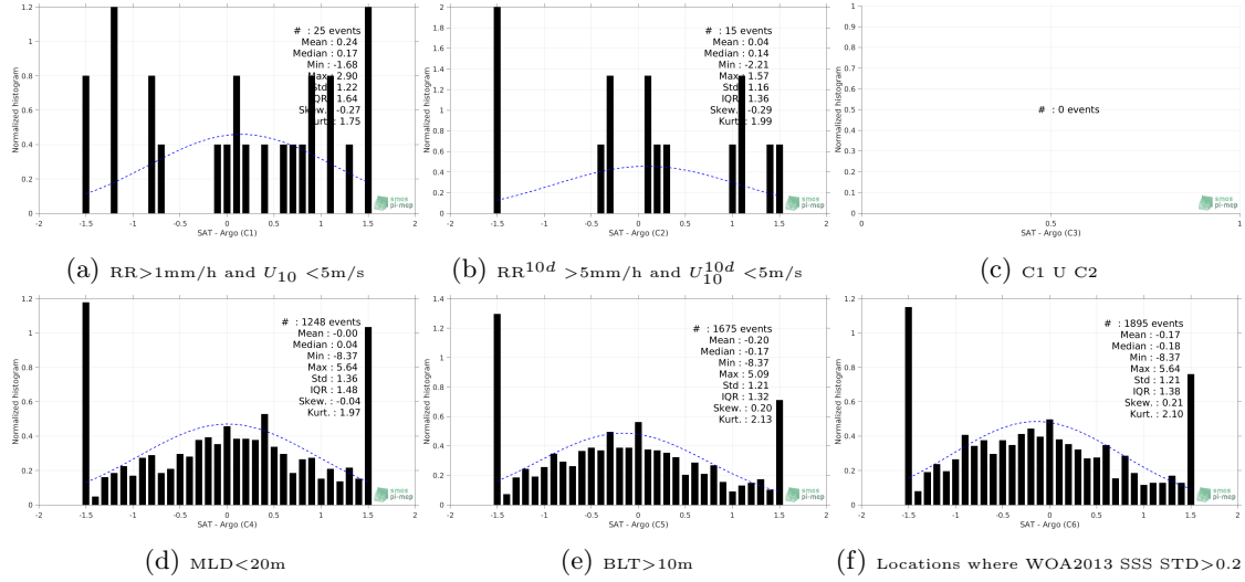
Figure 13: Normalized histogram of \Delta SSS (SMOS-L3-CATDS-CECOS-IFREMER-V2-1DAY-0.5DEG - Argo) for 6 different subdatasets corresponding to: RR > 1\text{mm/h} and U_{10} < 5\text{m/s} (a), RR^{10d} > 5\text{mm/h} and U_{10}^{10d} < 5\text{m/s} (b), C1 U C2 (c), MLD < 20\text{m} (d), BLT > 10\text{m} (e), Locations where WOA2013 SSS STD > 0.2 (f).
