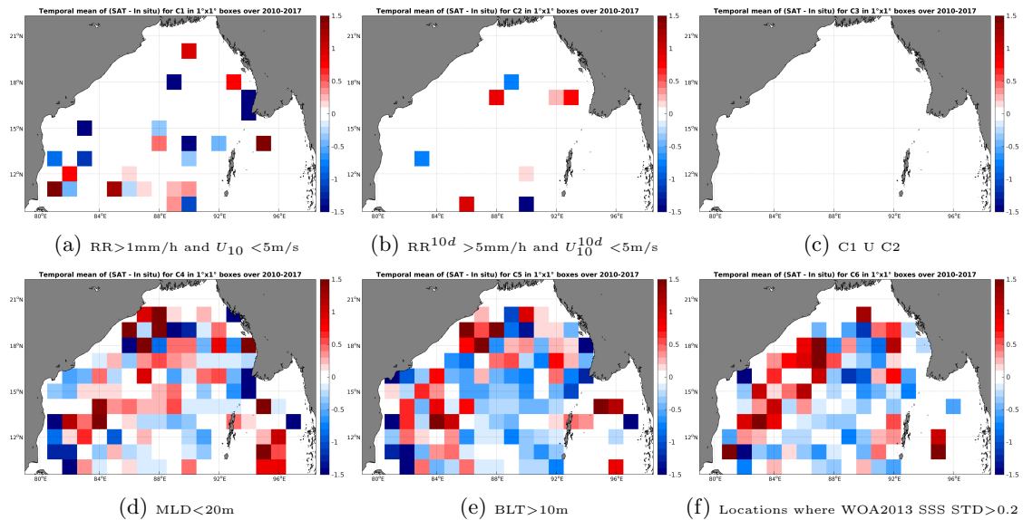
Figure 12: Temporal mean gridded over spatial boxes of size 1^\circ \times 1^\circ of \Delta SSS (SMOS-L3-CATDS-CECOS-IFREMER-V2-1DAY-0.5DEG - Argo) for 6 different subdatasets corresponding to: RR > 1mm/h and U_{10} < 5\text{m/s} (a), RR^{10d} > 5\text{mm/h} and U_{10}^{10d} < 5\text{m/s} (b), C1 U C2 (c), MLD < 20m (d), BLT > 10m (e), Locations where WOA2013 SSS STD > 0.2 (f).
