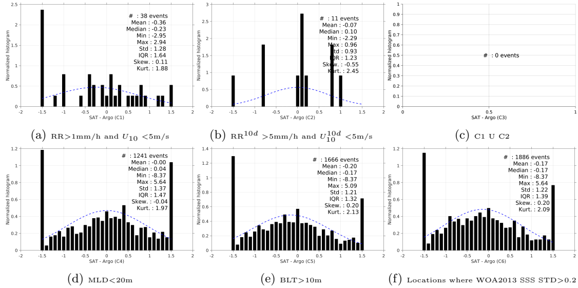
Figure 13: Normalized histogram of \Delta SSS (SMOS-L3-CATDS-CECOS-IFREMER-V2-1DAY-0.5deg - Argo) for 6 different subdatasets corresponding to: RR>1mm/h and U_{10} < 5\text{m/s} (a), RR^{10d} > 5\text{mm/h} and U_{10}^{10d} < 5\text{m/s} (b), C1 U C2 (c),MLD<20m (d),BLT>10m (e),Locations where WOA2013 SSS STD>0.2 (f).
