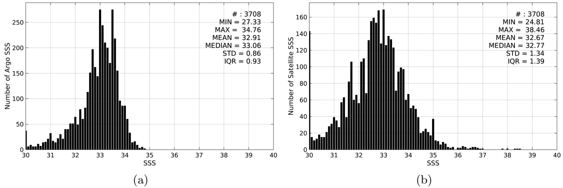
Figure 2: Histograms of SSS from Argo (a) and SMOS-L3-CATDS-CECOS-IFREMER-V2-1DAY-0.5deg (b) considering all match-up pairs per bins of 0.1 over the Bay of Bengal Pi-MEP region and for the full satellite product period.
