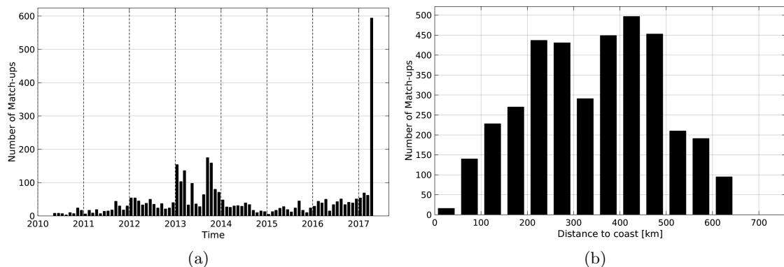
Figure 1: Number of match-ups between Argo and SMOS-L3-CATDS-CECOS-IFREMER-V2-1DAY-0.5deg SSS as a function of time (a) and as function of the distance to coast (b) over the Bay of Bengal Pi-MEP region and for the full satellite product period.
