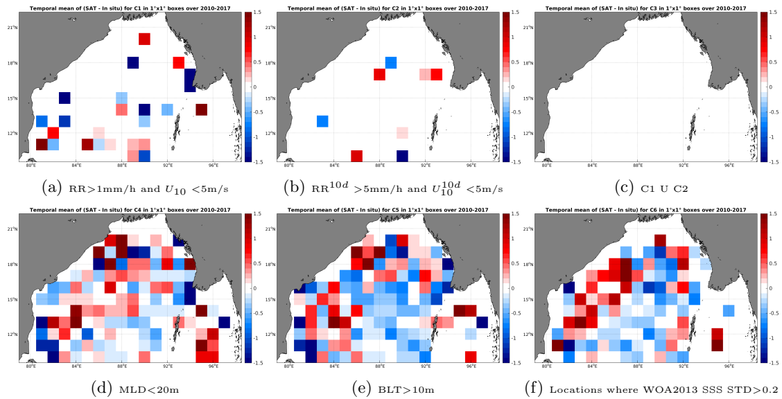
Figure 12: Temporal mean gridded over spatial boxes of size 1^\circ \times 1^\circ of \Delta SSS (SMOS-L3-CATDS-CECOS-IFREMER-V2-1DAY-0.5deg - Argo) for 6 different subdatasets corresponding to: RR > 1\text{mm/h} and U_{10} < 5\text{m/s} (a), RR^{10d} > 5\text{mm/h} and U_{10}^{10d} < 5\text{m/s} (b), C1 U C2 (c), MLD < 20\text{m} (d), BLT > 10\text{m} (e), Locations where WOA2013 SSS STD > 0.2 (f).
