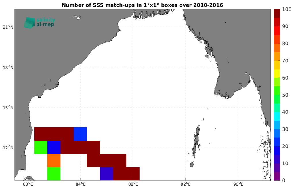
Figure 5: Number of SSS match-ups between TSG (LEGOS-DM) SSS and the SMOS SSS L3 v335 - Monthly - 25 km (CATDS-CPDC) SSS product for the Bay of Bengal Pi-MEP region over 1^\circ \times 1^\circ boxes and for the full satellite product period.
