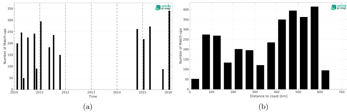
Figure 2: Number of match-ups between TSG (LEGOS-DM) and SMOS SSS L3 v335 - Monthly - 25 km (CATDS-CPDC) SSS as a function of time (a) and as function of the distance to coast (b) over the Bay of Bengal Pi-MEP region and for the full satellite product period.
