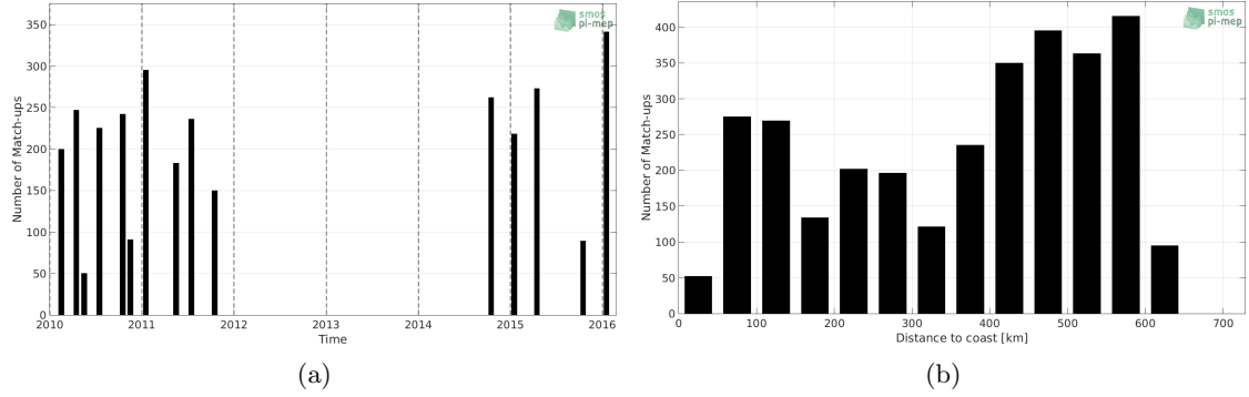
Figure 1: Number of match-ups between TSG (LEGOS-DM) and SMOS SSS L3 v335 - Monthly - 25 km (CATDS-CPDC) SSS as a function of time (a) and as function of the distance to coast (b) over the Bay of Bengal Pi-MEP region and for the full satellite product period.
