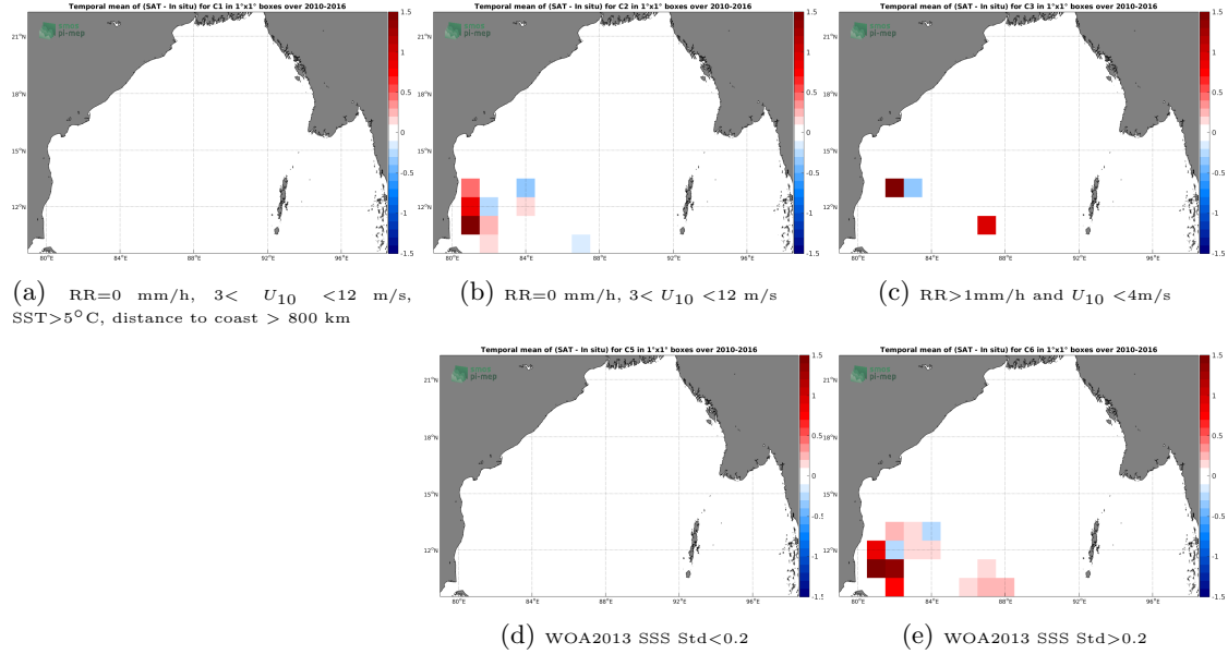
Figure 12: Temporal mean gridded over spatial boxes of size 1^{\circ}\times 1^{\circ} of \Delta\text{SSS} (SMOS SSS L3 v335 - Monthly - 25 km (CATDS-CPDC) - TSG (LEGOS-DM)) for 5 different subdatasets corresponding to: RR=0 mm/h, 3 < U_{10} < 12 m/s, SST > 5^{\circ}\text{C} , distance to coast > 800 km (a), RR=0 mm/h, 3 < U_{10} < 12 m/s (b), RR > 1 mm/h and U_{10} < 4 m/s (c), WOA2013 SSS Std < 0.2 (d), WOA2013 SSS Std > 0.2 (e).
