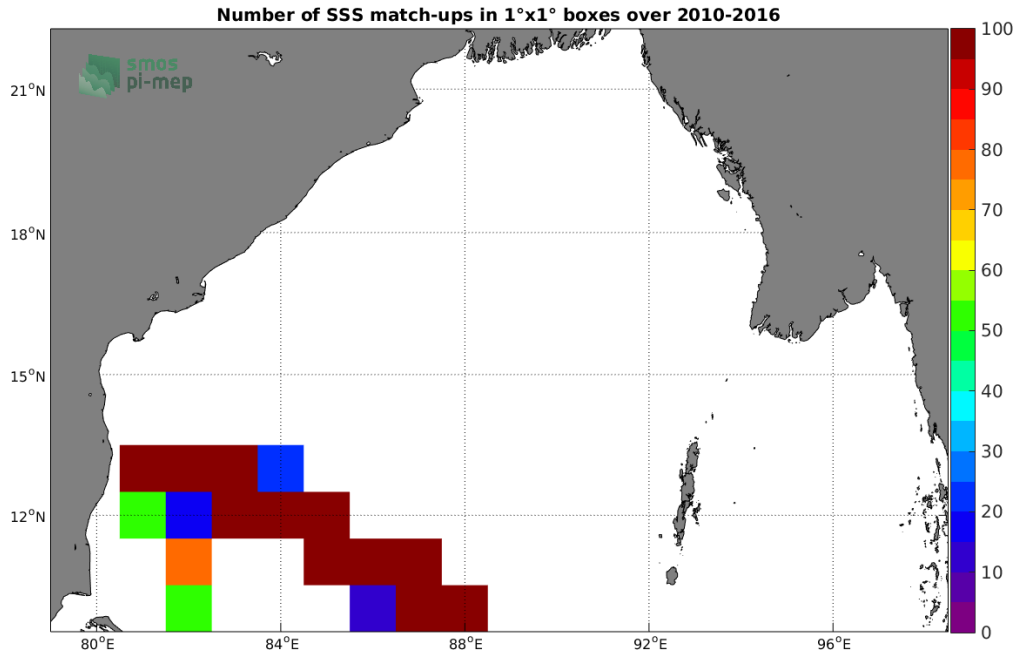
Figure 4: Number of SSS match-ups between TSG (LEGOS-DM) SSS and the SMOS SSS L3 v335 - Monthly - 25 km (CATDS-CPDC) SSS product for the Bay of Bengal Pi-MEP region over 1^\circ \times 1^\circ boxes and for the full satellite product period.
