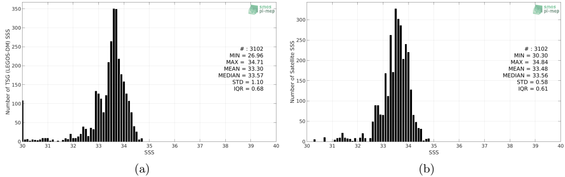
Figure 2: Histograms of SSS from TSG (LEGOS-DM) (a) and SMOS SSS L3 v335 - Monthly - 25 km (CATDS-CPDC) (b) considering all match-up pairs per bins of 0.1 over the Bay of Bengal Pi-MEP region and for the full satellite product period.
