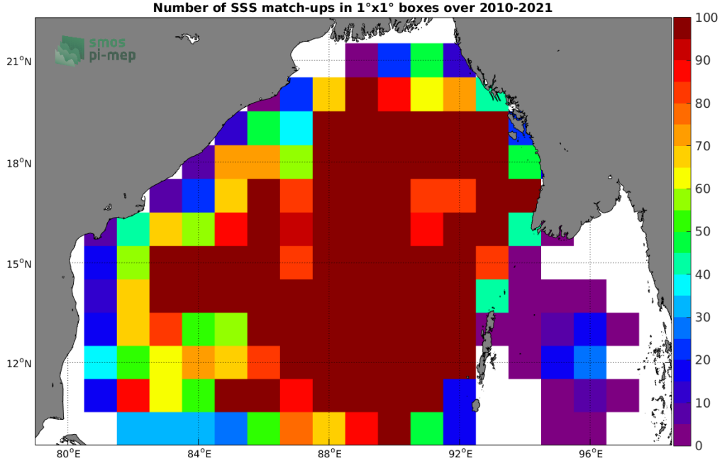
Figure 4: Number of SSS match-ups between Argo SSS and the SMOS SSS L3 v335 - Monthly - 25 km (CATDS-CPDC) SSS product for the Bay of Bengal Pi-MEP region over 1^\circ \times 1^\circ boxes and for the full satellite product period.
