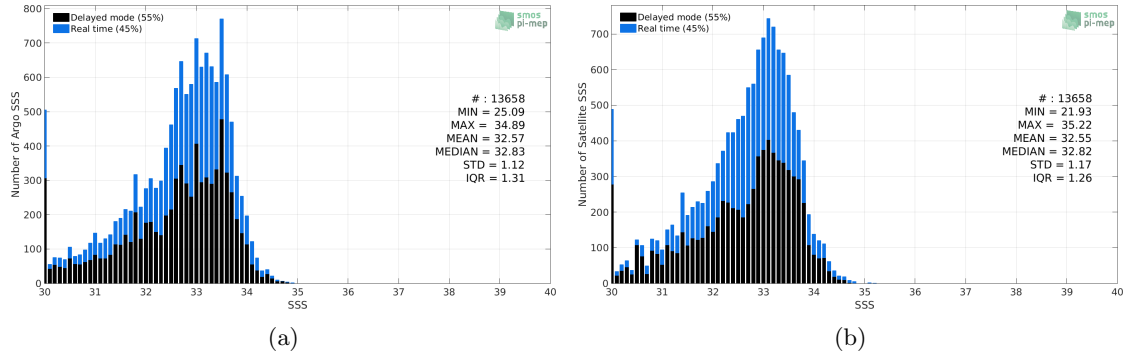
Figure 2: Histograms of SSS from Argo (a) and SMOS SSS L3 v335 - Monthly - 25 km (CATDS-CPDC) (b) considering all match-up pairs per bins of 0.1 over the Bay of Bengal Pi-MEP region and for the full satellite product period.
