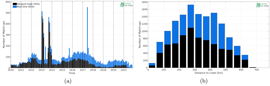
Figure 1: Number of match-ups between Argo and SMOS SSS L3 v335 - Monthly - 25 km (CATDS-CPDC) SSS as a function of time (a) and as function of the distance to coast (b) over the Bay of Bengal Pi-MEP region and for the full satellite product period.
