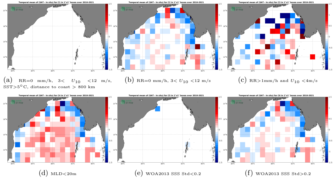
Figure 12: Temporal mean gridded over spatial boxes of size 1^\circ \times 1^\circ of \Delta SSS (SMOS SSS L3 v335 - Monthly - 25 km (CATDS-CPDC) - Argo) for 6 different subdatasets corresponding to: RR=0 mm/h, 3 < U_{10} < 12 m/s, SST > 5^\circ C , distance to coast > 800 km (a), RR=0 mm/h, 3 < U_{10} < 12 m/s (b), RR > 1 mm/h and U_{10} < 4 m/s (c), MLD < 20 m (d), WOA2013 SSS Std < 0.2 (e), WOA2013 SSS Std > 0.2 (f).
