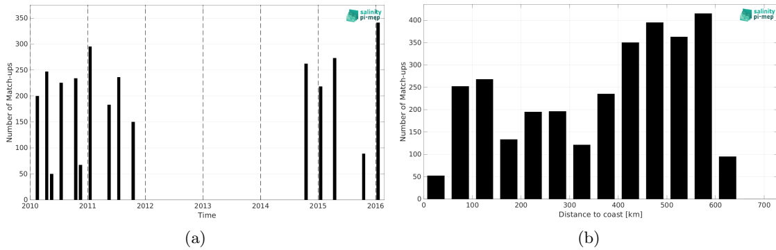
Figure 2: Number of match-ups between TSG (LEGOS-DM) and SMOS SSS L3 v335 - 10 Days - 25 km (CATDS-CPDC) SSS as a function of time (a) and as function of the distance to coast (b) over the Bay of Bengal Pi-MEP region and for the full satellite product period.
