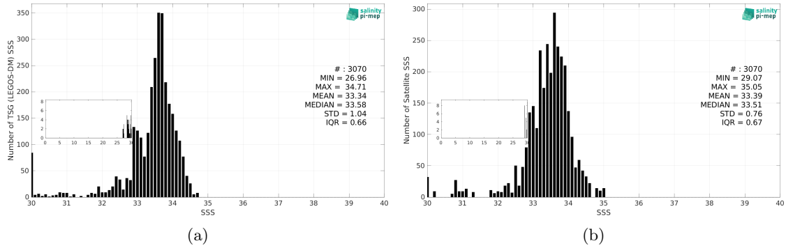
Figure 3: Histograms of SSS from TSG (LEGOS-DM) (a) and SMOS SSS L3 v335 - 10 Days - 25 km (CATDS-CPDC) (b) considering all match-up pairs per bins of 0.1 over the Bay of Bengal Pi-MEP region and for the full satellite product period.
