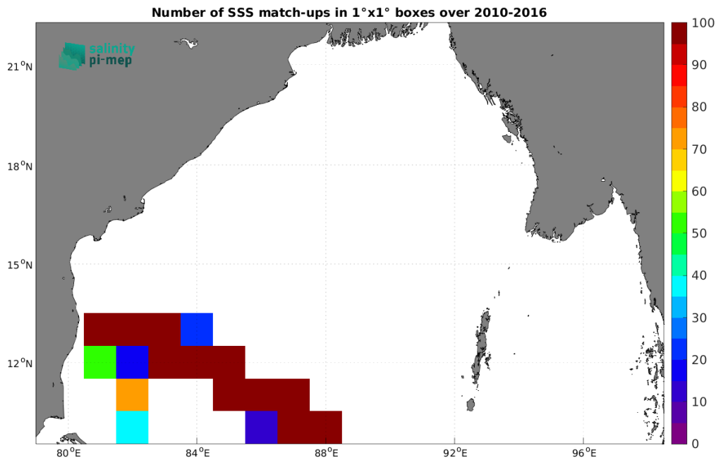
Figure 5: Number of SSS match-ups between TSG (LEGOS-DM) SSS and the SMOS SSS L3 v335 - 10 Days - 25 km (CATDS-CPDC) SSS product for the Bay of Bengal Pi-MEP region over 1^\circ \times 1^\circ boxes and for the full satellite product period.
