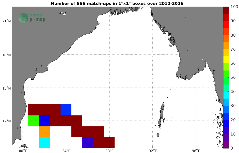
Figure 4: Number of SSS match-ups between TSG (LEGOS-DM) SSS and the SMOS SSS L3 v335 - 10 Days - 25 km (CATDS-CPDC) SSS product for the Bay of Bengal Pi-MEP region over 1^\circ \times 1^\circ boxes and for the full satellite product period.
