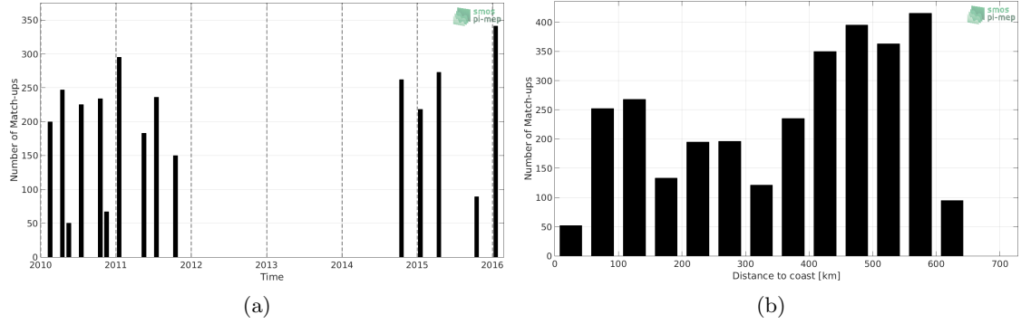
Figure 1: Number of match-ups between TSG (LEGOS-DM) and SMOS SSS L3 v335 - 10 Days - 25 km (CATDS-CPDC) SSS as a function of time (a) and as function of the distance to coast (b) over the Bay of Bengal Pi-MEP region and for the full satellite product period.
