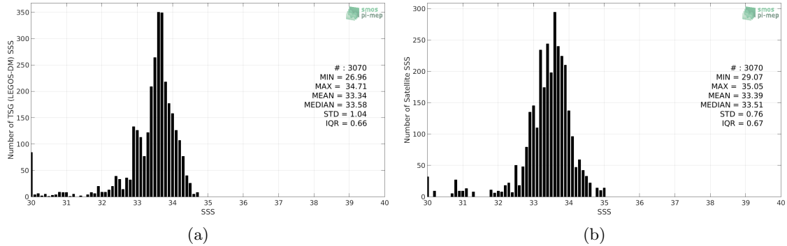
Figure 2: Histograms of SSS from TSG (LEGOS-DM) (a) and SMOS SSS L3 v335 - 10 Days - 25 km (CATDS-CPDC) (b) considering all match-up pairs per bins of 0.1 over the Bay of Bengal Pi-MEP region and for the full satellite product period.
