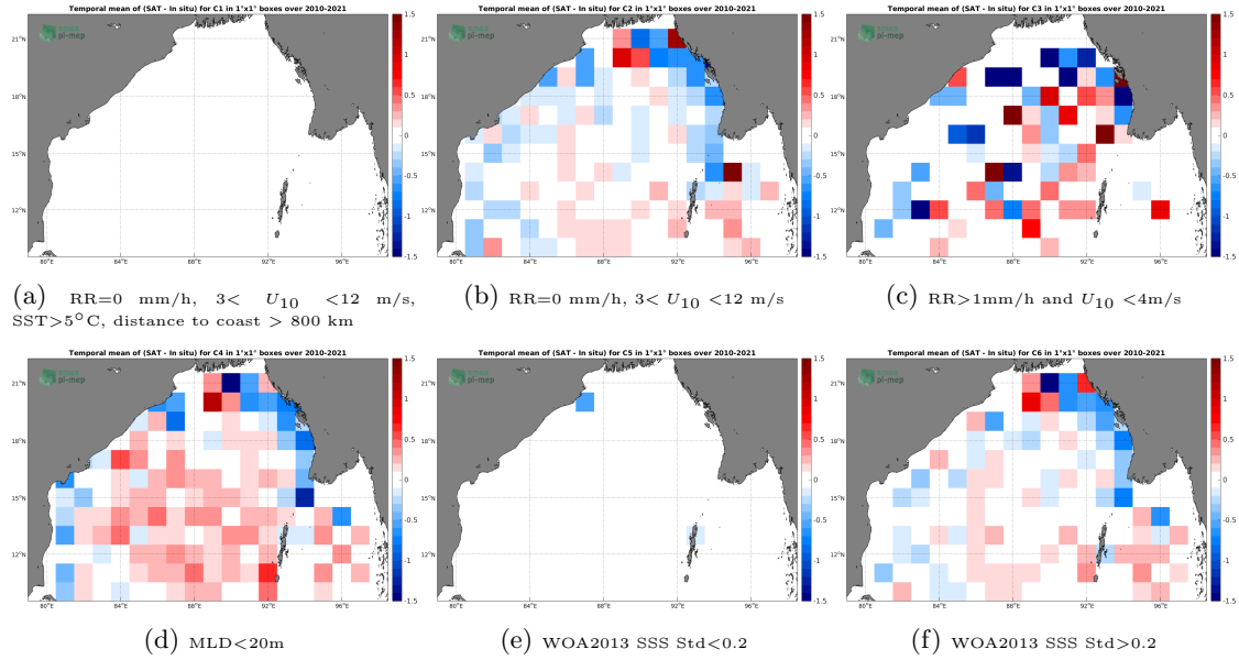
Figure 12: Temporal mean gridded over spatial boxes of size 1^\circ \times 1^\circ of \Delta SSS (SMOS SSS L3 v335 - 10 Days - 25 km (CATDS-CPDC) - Argo) for 6 different subdatasets corresponding to: RR=0 mm/h, 3 < U_{10} < 12 m/s, SST > 5^\circ C , distance to coast > 800 km (a), RR=0 mm/h, 3 < U_{10} < 12 m/s (b), RR > 1 mm/h and U_{10} < 4 m/s (c), MLD < 20 m (d), WOA2013 SSS Std < 0.2 (e), WOA2013 SSS Std > 0.2 (f).
