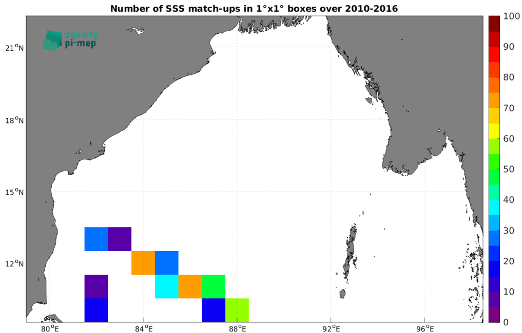
Figure 5: Number of SSS match-ups between TSG (LEGOS-DM) SSS and the SMOS SSS L2Q v333 - 0.25 Deg (CATDS-CPDC) SSS product for the Bay of Bengal Pi-MEP region over 1^\circ \times 1^\circ boxes and for the full satellite product period.
