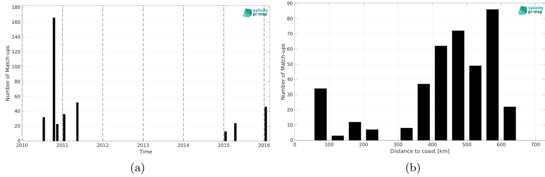
Figure 2: Number of match-ups between TSG (LEGOS-DM) and SMOS SSS L2Q v333 - 0.25 Deg (CATDS-CPDC) SSS as a function of time (a) and as function of the distance to coast (b) over the Bay of Bengal Pi-MEP region and for the full satellite product period.
