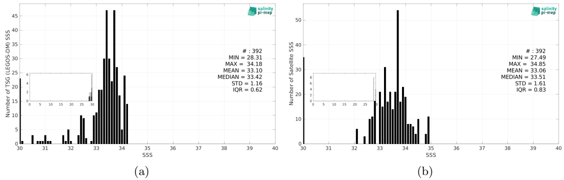
Figure 3: Histograms of SSS from TSG (LEGOS-DM) (a) and SMOS SSS L2Q v333 - 0.25 Deg (CATDS-CPDC) (b) considering all match-up pairs per bins of 0.1 over the Bay of Bengal Pi-MEP region and for the full satellite product period.
