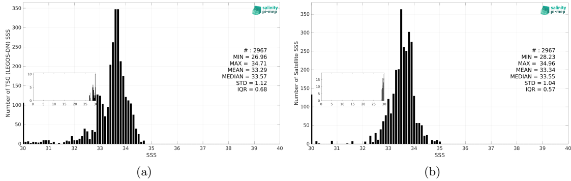
Figure 3: Histograms of SSS from TSG (LEGOS-DM) (a) and SMOS SSS L3 v332 - 9 Days (CATDS-CPDC) (b) considering all match-up pairs per bins of 0.1 over the Bay of Bengal Pi-MEP region and for the full satellite product period.
