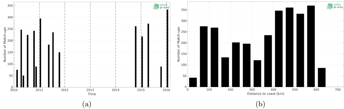
Figure 1: Number of match-ups between TSG (LEGOS-DM) and SMOS SSS L3 v332 - 9 Days (CATDS-CPDC) SSS as a function of time (a) and as function of the distance to coast (b) over the Bay of Bengal Pi-MEP region and for the full satellite product period.
