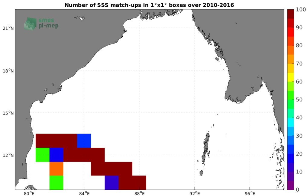
Figure 4: Number of SSS match-ups between TSG (LEGOS-DM) SSS and the SMOS SSS L3 v332 - 9 Days (CATDS-CPDC) SSS product for the Bay of Bengal Pi-MEP region over 1^\circ \times 1^\circ boxes and for the full satellite product period.
