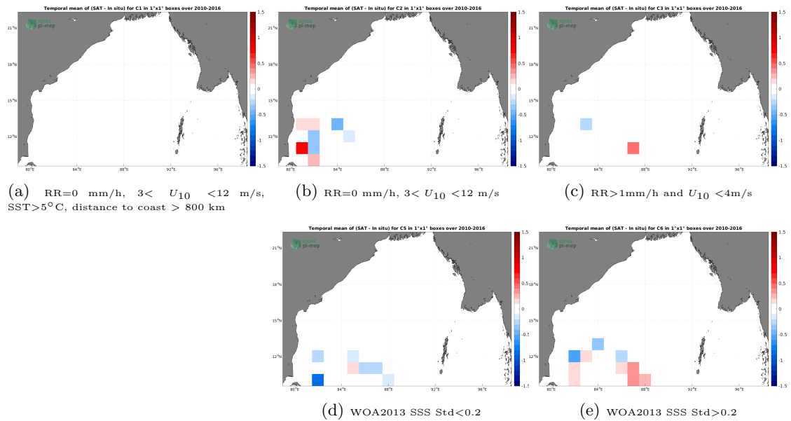
Figure 12: Temporal mean gridded over spatial boxes of size 1^\circ \times 1^\circ of \Delta SSS (SMOS SSS L3 v332 - 9 Days (CATDS-CPDC) - TSG (LEGOS-DM)) for 5 different subdatasets corresponding to:RR=0 mm/h, 3 < U_{10} < 12 m/s, SST >5^\circ\text{C} , distance to coast > 800 km (a), RR=0 mm/h, 3 < U_{10} < 12 m/s (b), RR >1 mm/h and U_{10} < 4 m/s (c), WOA2013 SSS Std <0.2 (d), WOA2013 SSS Std >0.2 (e).
