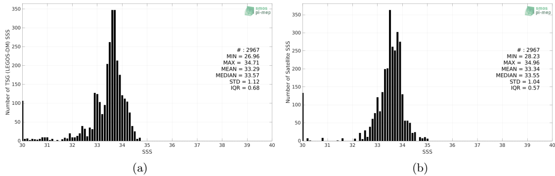
Figure 2: Histograms of SSS from TSG (LEGOS-DM) (a) and SMOS SSS L3 v332 - 9 Days (CATDS-CPDC) (b) considering all match-up pairs per bins of 0.1 over the Bay of Bengal Pi-MEP region and for the full satellite product period.
