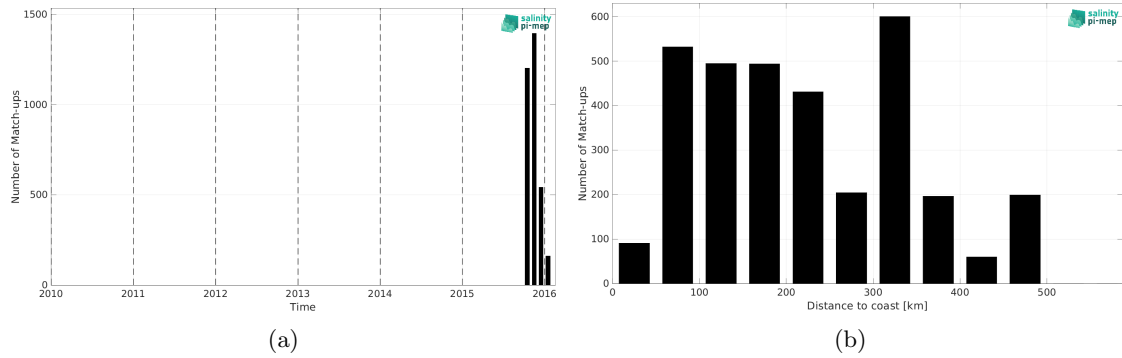
Figure 2: Number of match-ups between Surface drifters and SMOS SSS L3 v332 - 9 Days (CATDS-CPDC) SSS as a function of time (a) and as function of the distance to coast (b) over the Bay of Bengal Pi-MEP region and for the full satellite product period.
