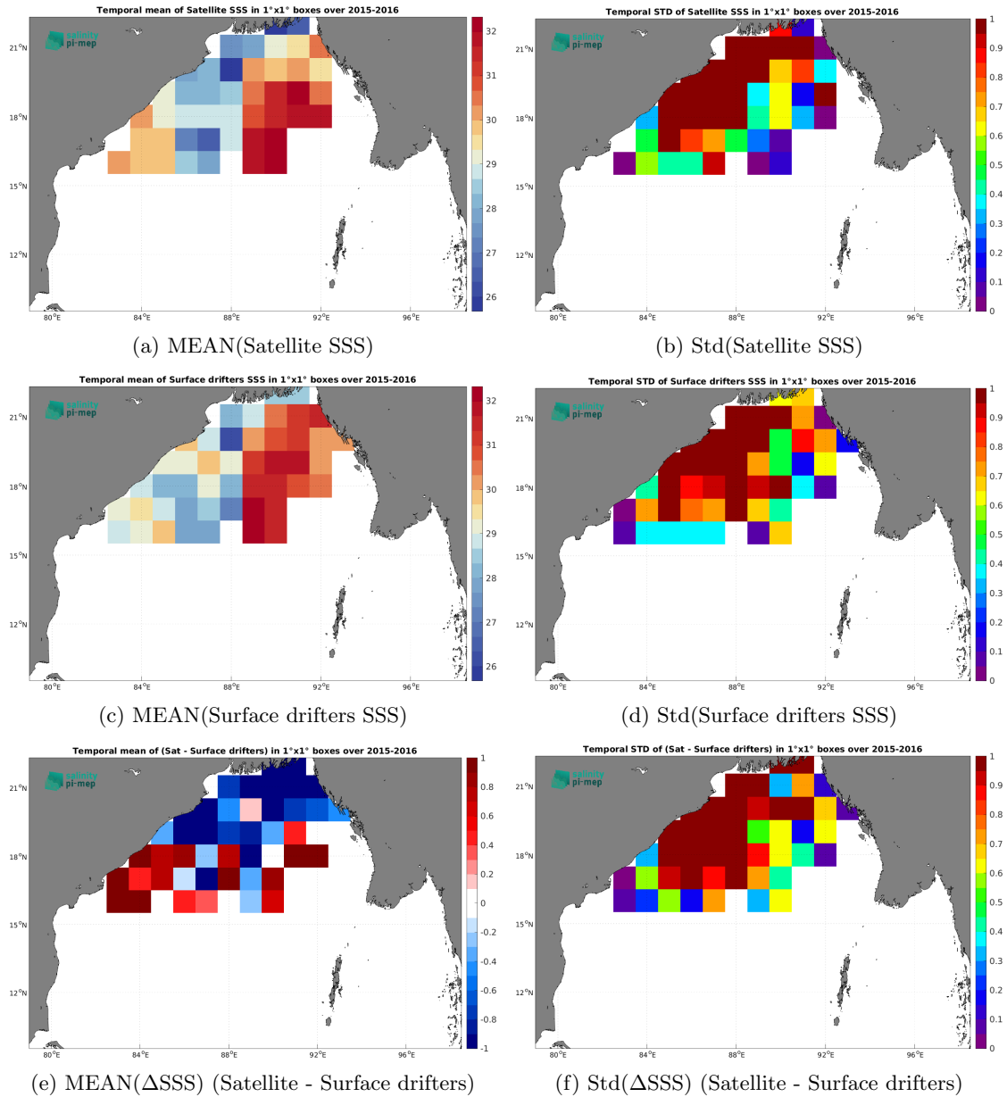
Figure 6: Temporal mean (left) and Std (right) of SSS from SMOS SSS L3 v332 - 9 Days (CATDS-CPDC) (top), Surface drifters (middle), and of \Delta SSS (Satellite - Surface drifters). Only match-up pairs are used to generate these maps.
