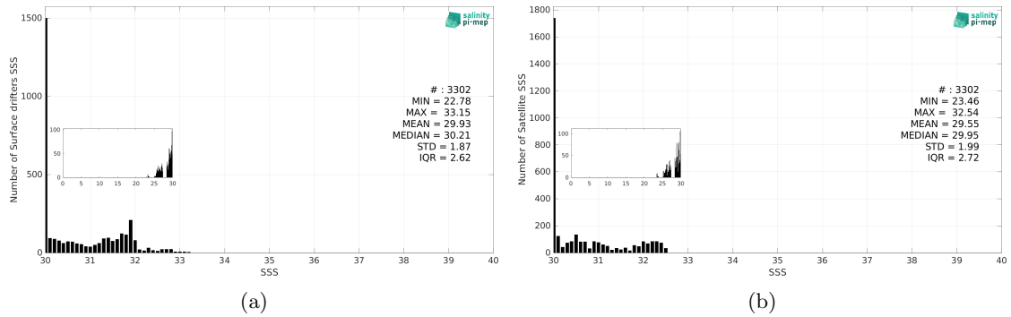
Figure 3: Histograms of SSS from Surface drifters (a) and SMOS SSS L3 v332 - 9 Days (CATDS-CPDC) (b) considering all match-up pairs per bins of 0.1 over the Bay of Bengal Pi-MEP region and for the full satellite product period.
