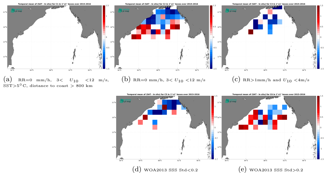
Figure 13: Temporal mean gridded over spatial boxes of size 1^\circ \times 1^\circ of \Delta SSS (SMOS SSS L3 v332 - 9 Days (CATDS-CPDC) - Surface drifters) for 5 different subdatasets corresponding to:RR=0 mm/h, 3 < U_{10} < 12 m/s, SST > 5^\circ\text{C} , distance to coast > 800 km (a), RR=0 mm/h, 3 < U_{10} < 12 m/s (b), RR > 1 mm/h and U_{10} < 4 m/s (c), WOA2013 SSS Std < 0.2 (d), WOA2013 SSS Std > 0.2 (e).
