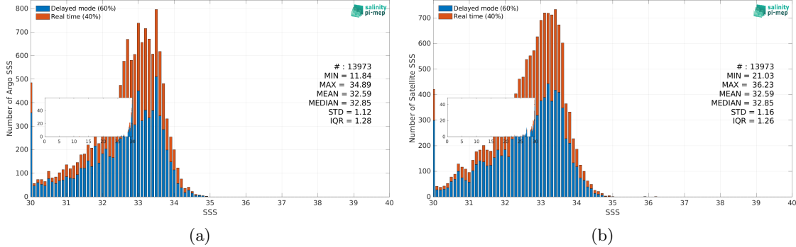
Figure 3: Histograms of SSS from Argo (a) and SMOS SSS L3 v332 - 9 Days (CATDS-CPDC) (b) considering all match-up pairs per bins of 0.1 over the Bay of Bengal Pi-MEP region and for the full satellite product period.
