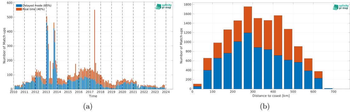
Figure 2: Number of match-ups between Argo and SMOS SSS L3 v332 - 9 Days (CATDS-CPDC) SSS as a function of time (a) and as function of the distance to coast (b) over the Bay of Bengal Pi-MEP region and for the full satellite product period.
