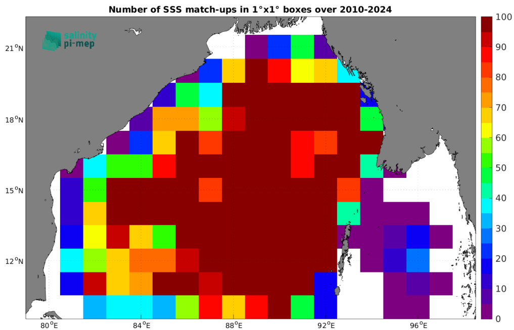
Figure 5: Number of SSS match-ups between Argo SSS and the SMOS SSS L3 v332 - 9 Days (CATDS-CPDC) SSS product for the Bay of Bengal Pi-MEP region over 1^\circ \times 1^\circ boxes and for the full satellite product period.
