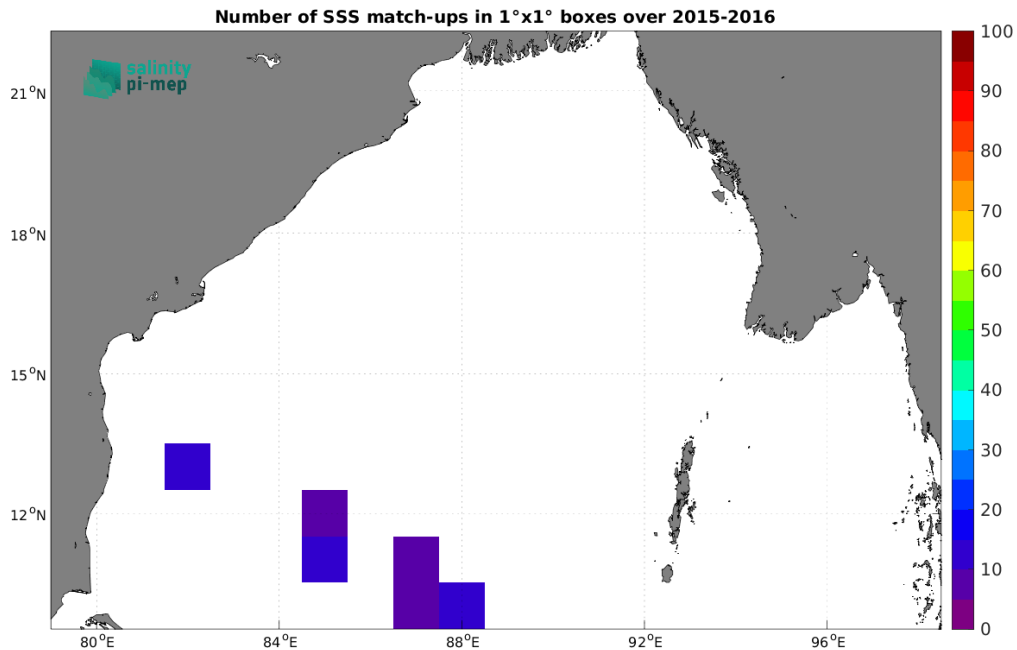
Figure 4: Number of SSS match-ups between TSG (LEGOS-DM) SSS and the SMOS SSS L2Q v331 - 0.25 Deg (CATDS-CPDC) SSS product for the Bay of Bengal Pi-MEP region over 1^\circ \times 1^\circ boxes and for the full satellite product period.
