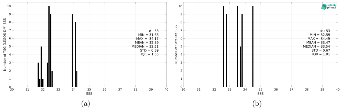
Figure 2: Histograms of SSS from TSG (LEGOS-DM) (a) and SMOS SSS L2Q v331 - 0.25 Deg (CATDS-CPDC) (b) considering all match-up pairs per bins of 0.1 over the Bay of Bengal Pi-MEP region and for the full satellite product period.
