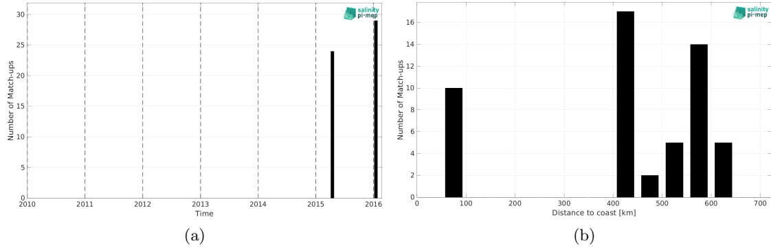
Figure 1: Number of match-ups between TSG (LEGOS-DM) and SMOS SSS L2Q v331 - 0.25 Deg (CATDS-CPDC) SSS as a function of time (a) and as function of the distance to coast (b) over the Bay of Bengal Pi-MEP region and for the full satellite product period.
