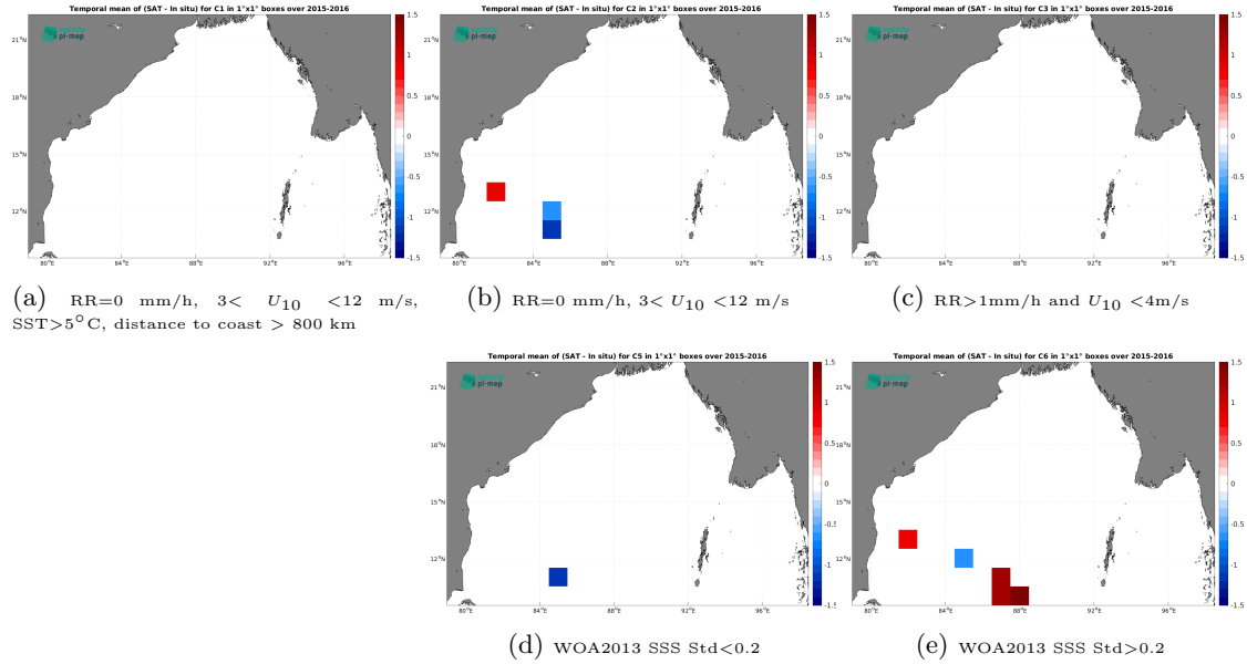
Figure 12: Temporal mean gridded over spatial boxes of size 1^{\circ}\times 1^{\circ} of \Delta\text{SSS} (SMOS SSS L2Q v331 - 0.25 Deg (CATDS-CPDC) - TSG (LEGOS-DM)) for 5 different subdatasets corresponding to:RR=0 mm/h, 3 < U_{10} < 12 m/s, SST > 5^{\circ}\text{C} , distance to coast > 800 km (a), RR=0 mm/h, 3 < U_{10} < 12 m/s (b), RR > 1 mm/h and U_{10} < 4 m/s (c), WOA2013 SSS Std < 0.2 (d), WOA2013 SSS Std > 0.2 (e).
