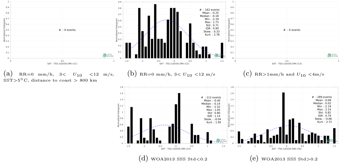
Figure 13: Normalized histogram of \Delta SSS (SMOS SSS L2Q v331 - 0.25 Deg (CATDS-CPDC) - TSG (LEGOS-DM)) for 5 different subdatasets corresponding to: RR=0 mm/h, 3 < U_{10} < 12 m/s, SST > 5°C, distance to coast > 800 km (a), RR=0 mm/h, 3 < U_{10} < 12 m/s (b), RR > 1mm/h and U_{10} < 4 m/s (c), WOA2013 SSS Std < 0.2 (d), WOA2013 SSS Std > 0.2 (e).
