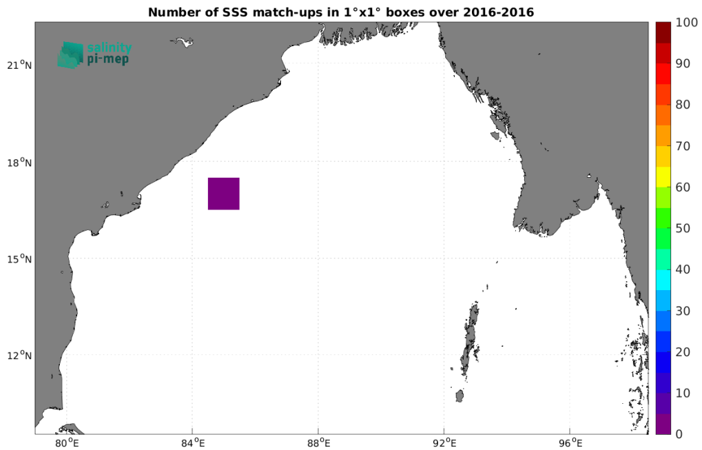
Figure 3: Number of SSS match-ups between Surface drifters SSS and the SMOS SSS L2Q v331 - 0.25 Deg (CATDS-CPDC) SSS product for the Bay of Bengal Pi-MEP region over 1°x1° boxes and for the full satellite product period.
