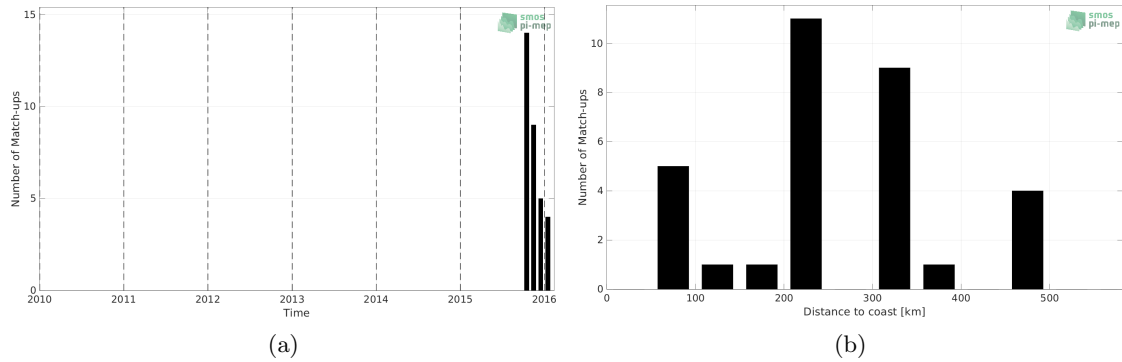
Figure 1: Number of match-ups between Surface drifters and SMOS SSS L2Q v331 - 0.25 Deg (CATDS-CPDC) SSS as a function of time (a) and as function of the distance to coast (b) over the Bay of Bengal Pi-MEP region and for the full satellite product period.
