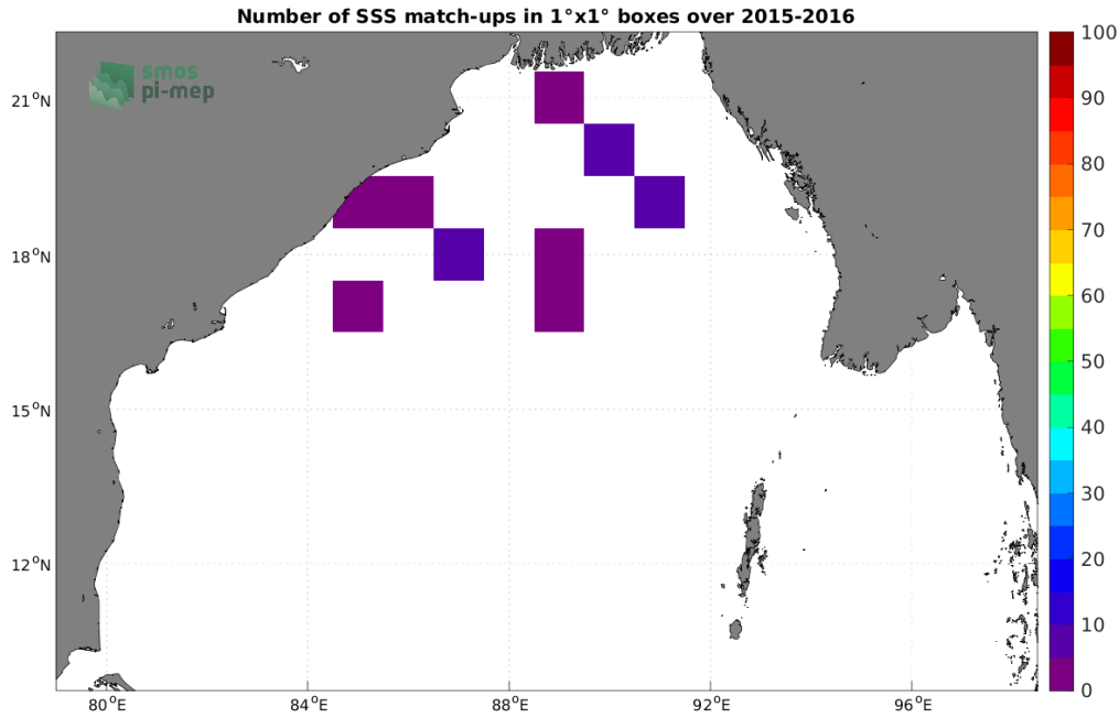
Figure 3: Number of SSS match-ups between Surface drifters SSS and the SMOS SSS L2Q v331 - 0.25 Deg (CATDS-CPDC) SSS product for the Bay of Bengal Pi-MEP region over 1° × 1° boxes and for the full satellite product period.
