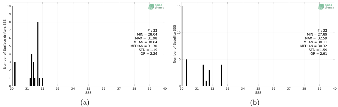
Figure 2: Histograms of SSS from Surface drifters (a) and SMOS SSS L2Q v331 - 0.25 Deg (CATDS-CPDC) (b) considering all match-up pairs per bins of 0.1 over the Bay of Bengal Pi-MEP region and for the full satellite product period.
