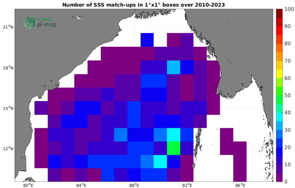
Figure 4: Number of SSS match-ups between Argo SSS and the SMOS SSS L2Q v331 - 0.25 Deg (CATDS-CPDC) SSS product for the Bay of Bengal Pi-MEP region over 1^\circ \times 1^\circ boxes and for the full satellite product period.
