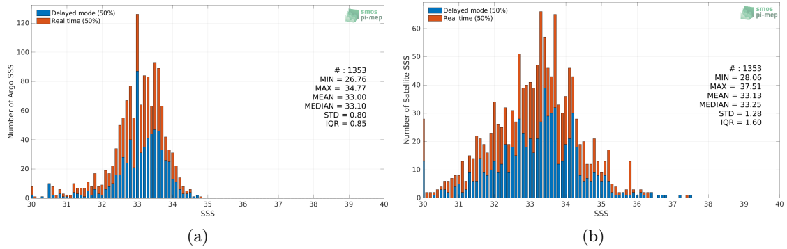
Figure 2: Histograms of SSS from Argo (a) and SMOS SSS L2Q v331 - 0.25 Deg (CATDS-CPDC) (b) considering all match-up pairs per bins of 0.1 over the Bay of Bengal Pi-MEP region and for the full satellite product period.
