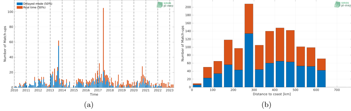
Figure 1: Number of match-ups between Argo and SMOS SSS L2Q v331 - 0.25 Deg (CATDS-CPDC) SSS as a function of time (a) and as function of the distance to coast (b) over the Bay of Bengal Pi-MEP region and for the full satellite product period.
